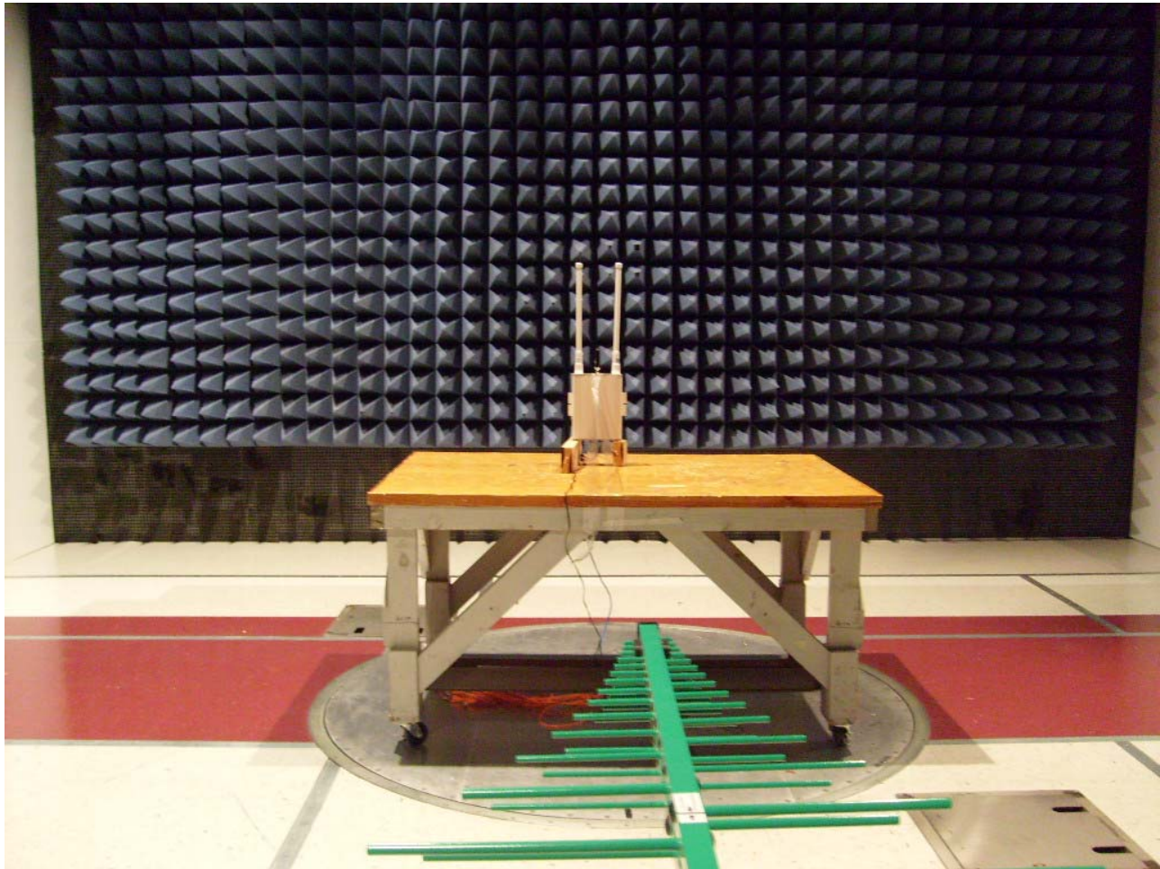
Photograph 1. Radiated Emission Limits Test Setup
