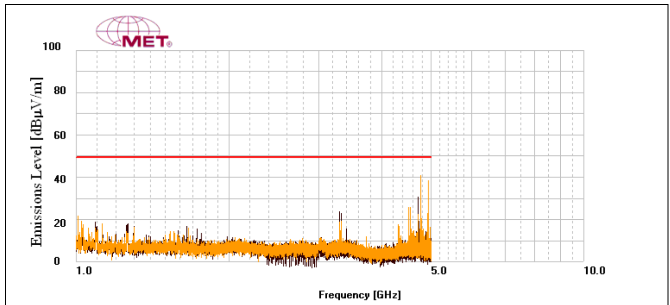
Radiated Emission, 1-5GHz Plot
