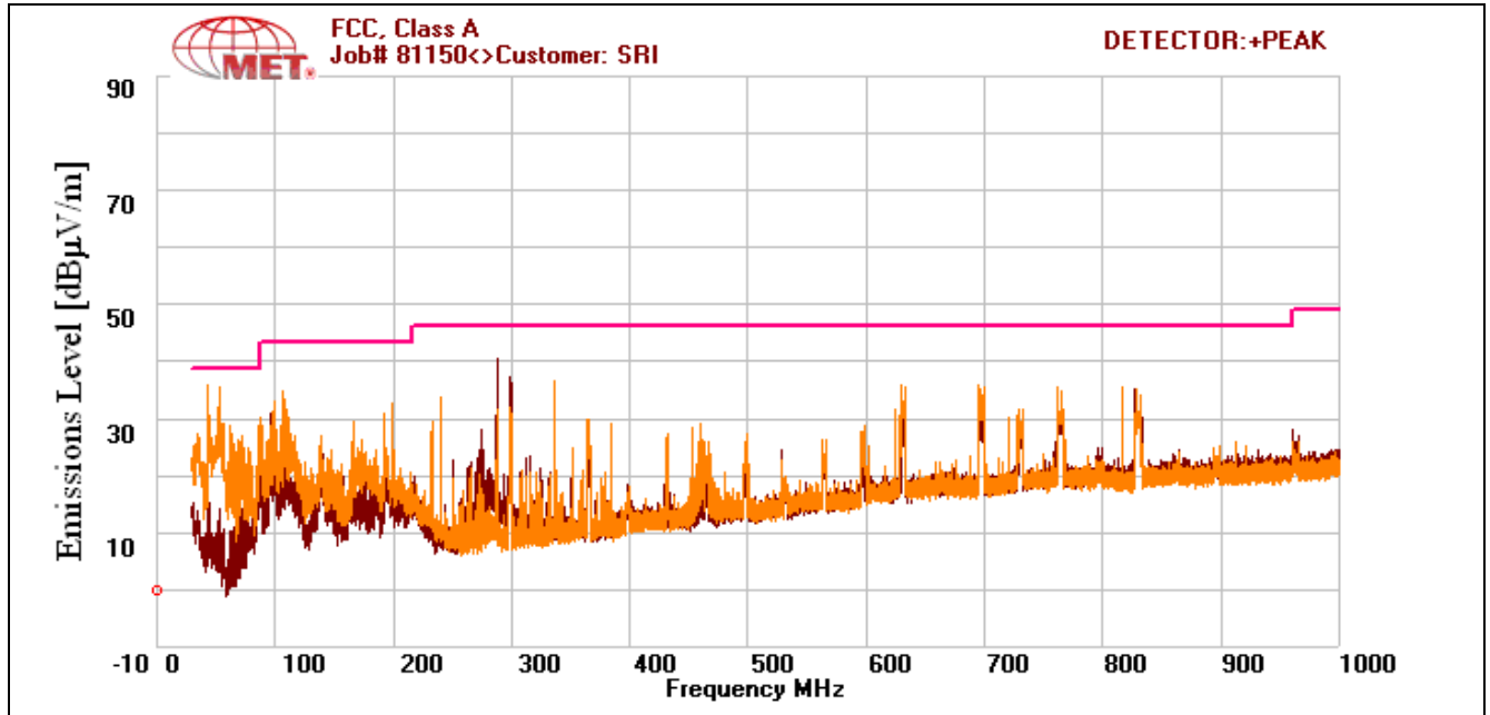
Radiated Emission, 30MHz-1GHz Plot
