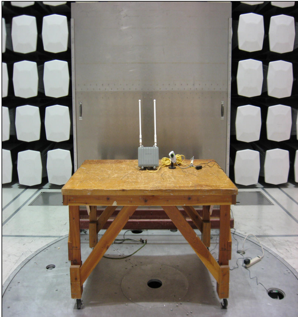
Photograph 1. Conducted Emissions Test Setup
