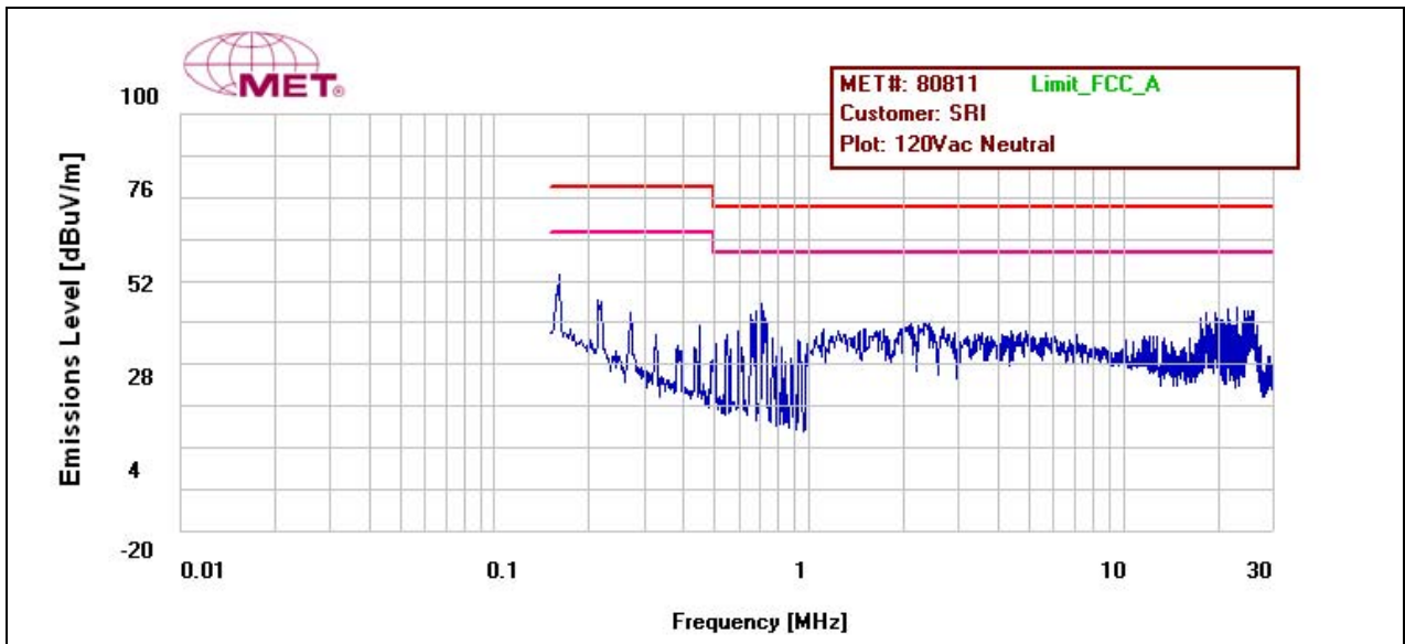
Conducted Emission, Neutral Line Plot 120Vac with Shielding
