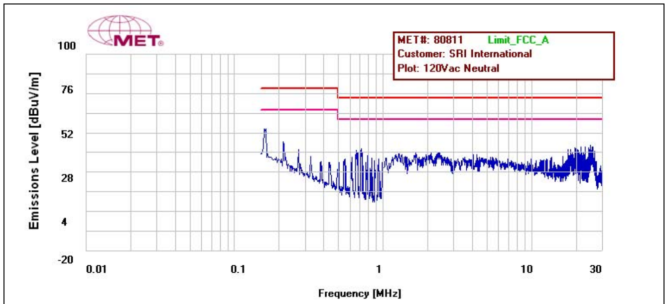
Conducted Emission, Neutral Line Plot, 120Vac without Shielding
