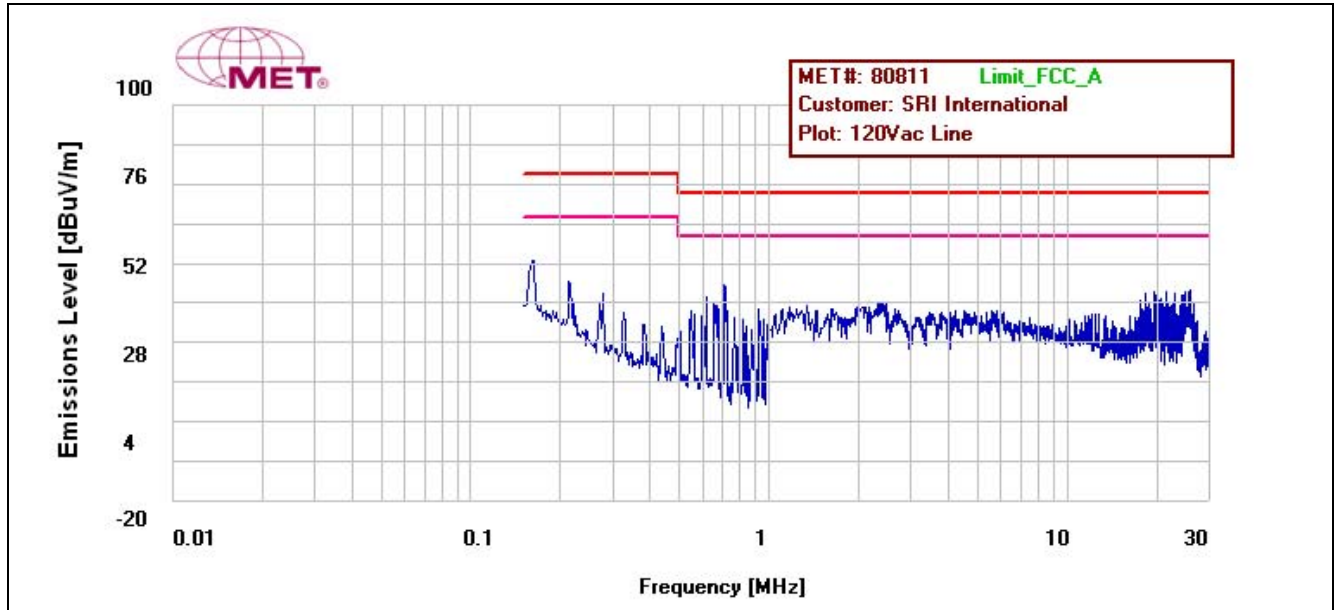
Conducted Emission, Phase Line Plot, 120Vac without Shielding
