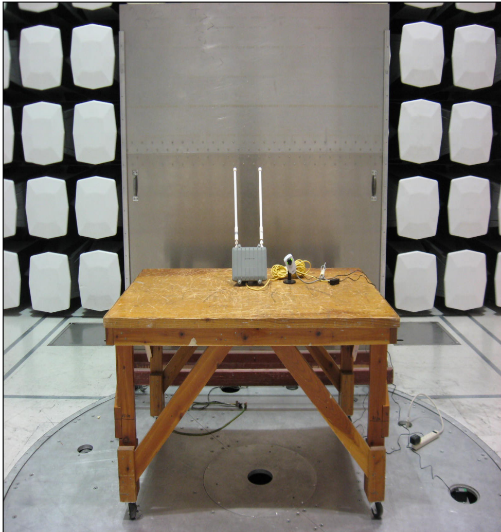
Photograph 1. Conducted Emissions Test Setup
