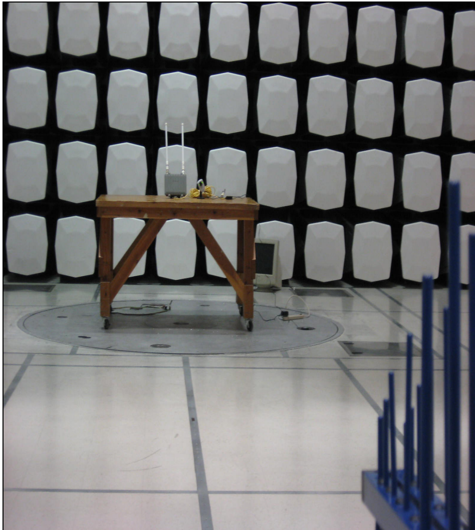
Photograph 2. Radiated Emission Limits Test Setup
