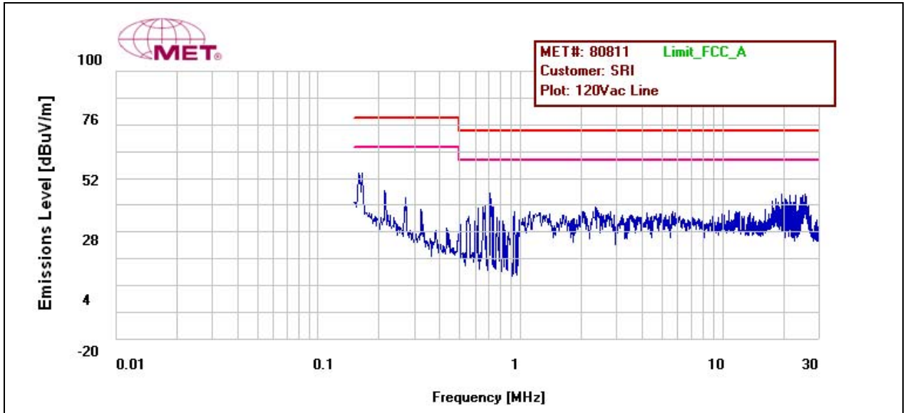
Conducted Emission, Phase Line Plot 120Vac with Shielding
