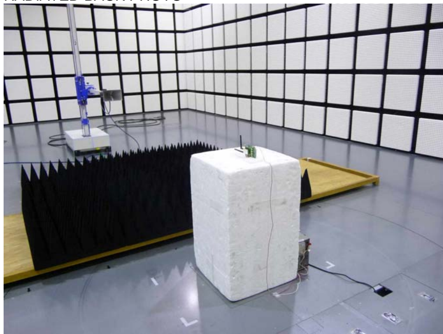
RADIATED BACK PHOTO
