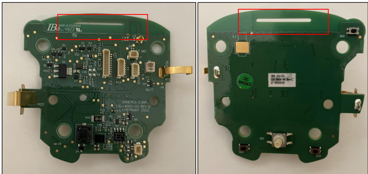
Figure 6 - Internal Photos – Left Side PCBA, Front and Back
