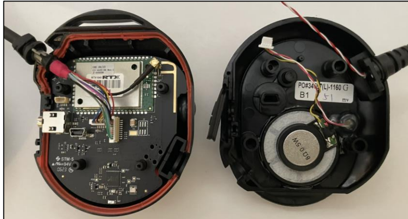
Figure 1 - Internal Photos – Right Side
