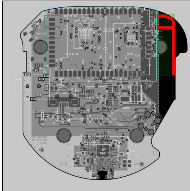
Figure 7 – Right Side PCBA – F Antenna Location
