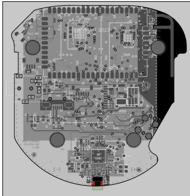
Figure 8 – Right Side PCBA – BT Antenna Location
