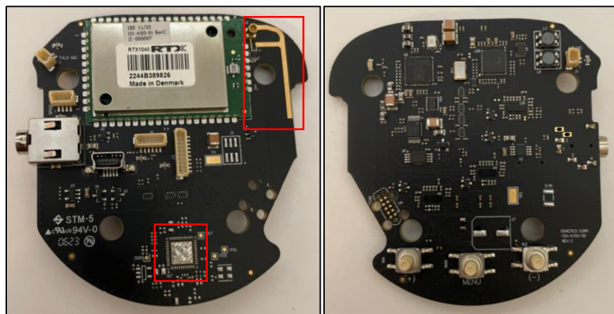
Figure 3 - Internal Photos – Right Side PCBA - No BT Module, Front and Back
