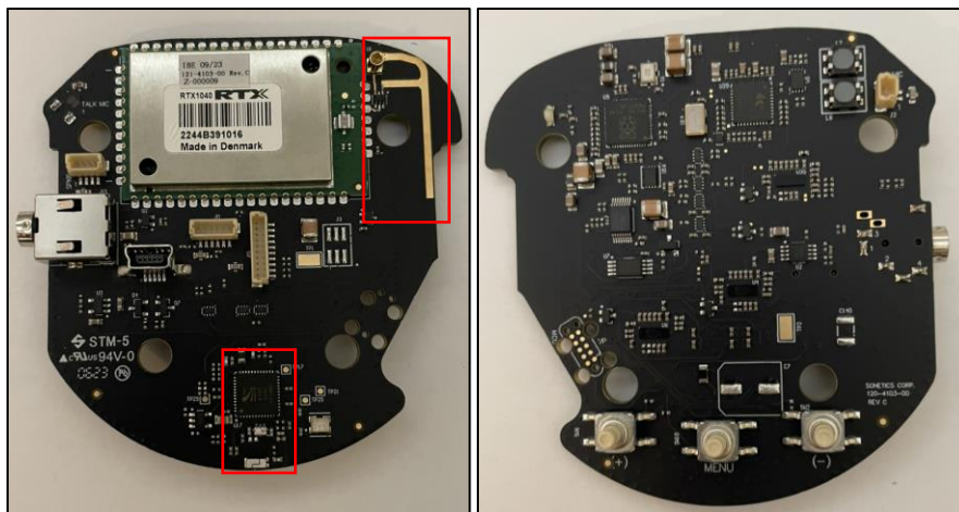
Figure 2 - Internal Photos – Right Side PCBA – BT Module, Front and Back
