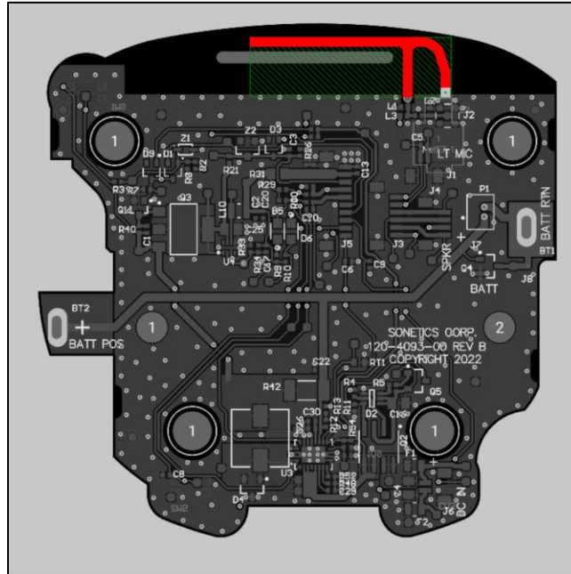
Figure 9 – Left Side PCBA – F Antenna Location
