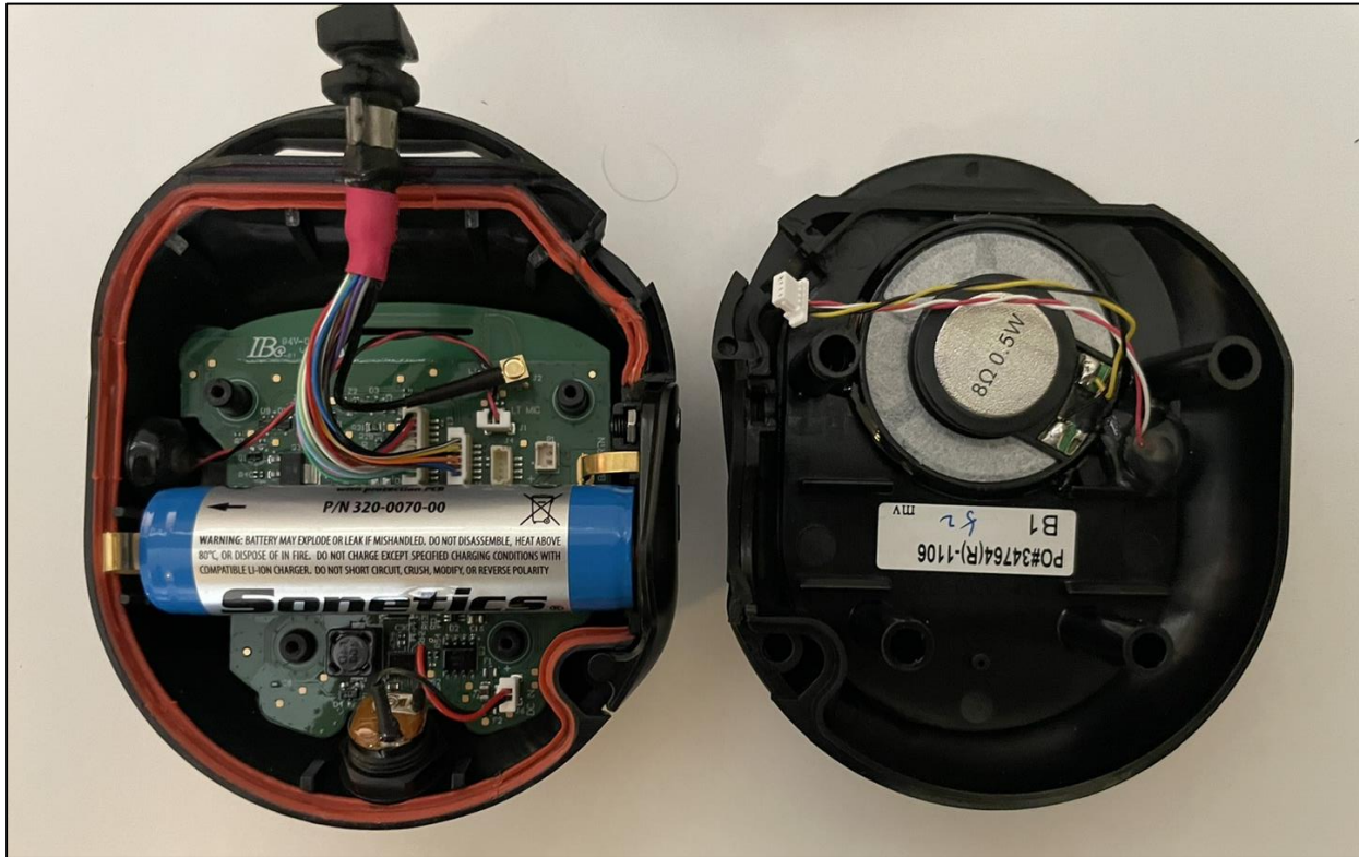
Figure 4 - Internal Photos – Left Side
