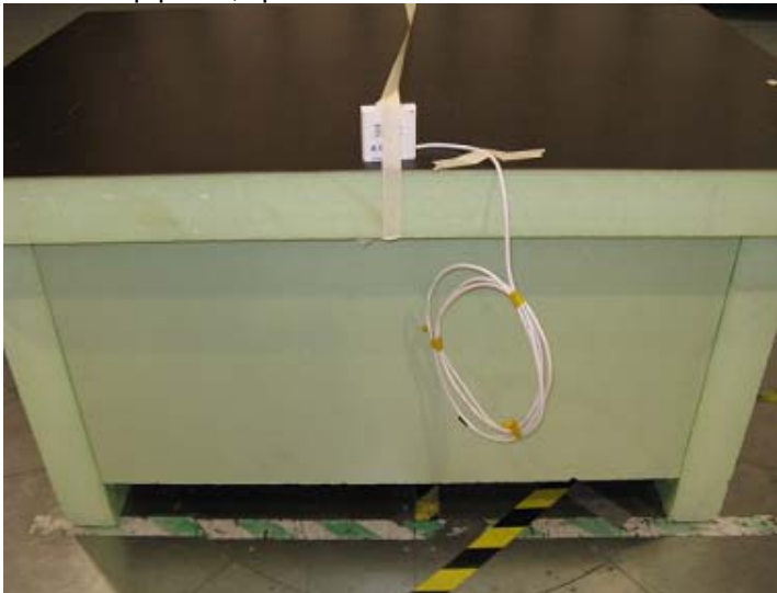
Test set-up photo, spurious emission 30-1000 MHz:
