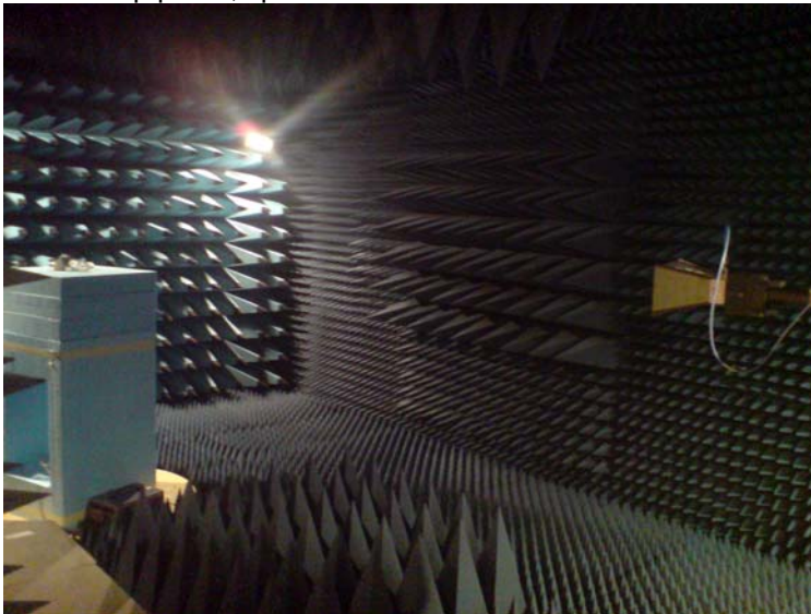
Test set-up photo, spurious emission 1-13 GHz:
