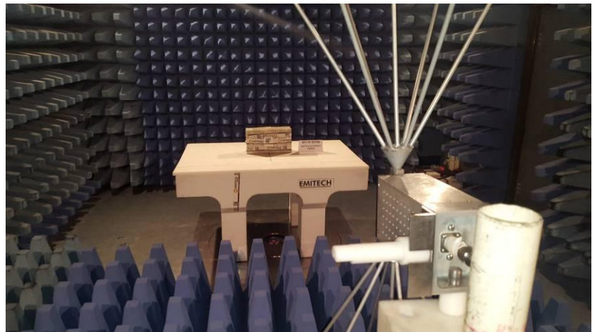
Radiated pre measurement Thermostat Digital
