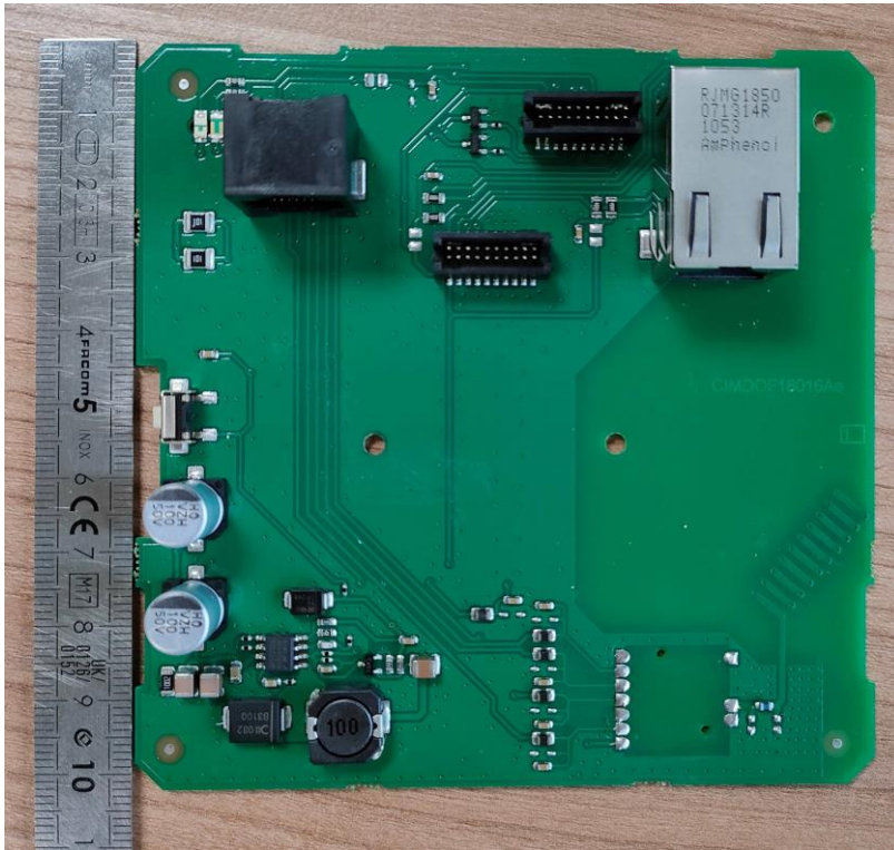
R208 NA – PCB Back view
