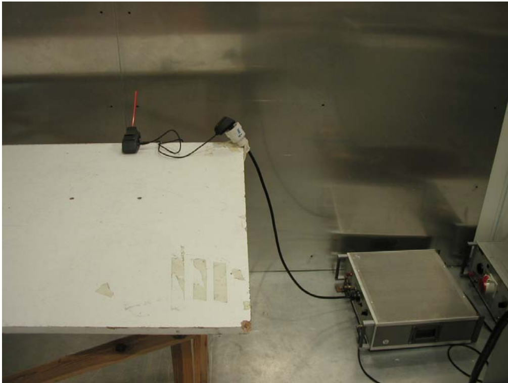
Photograph 5. AC power line conducted emissions test setup
