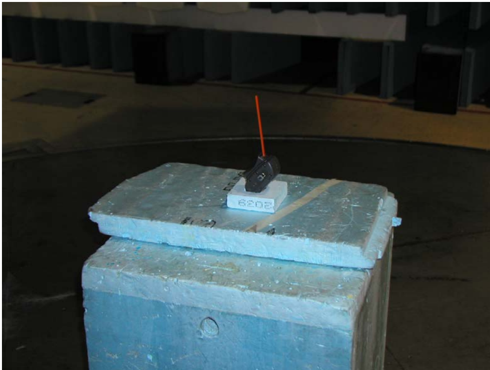
Photograph 1. Radiated RF output power and spurious radiated emissions test setup
