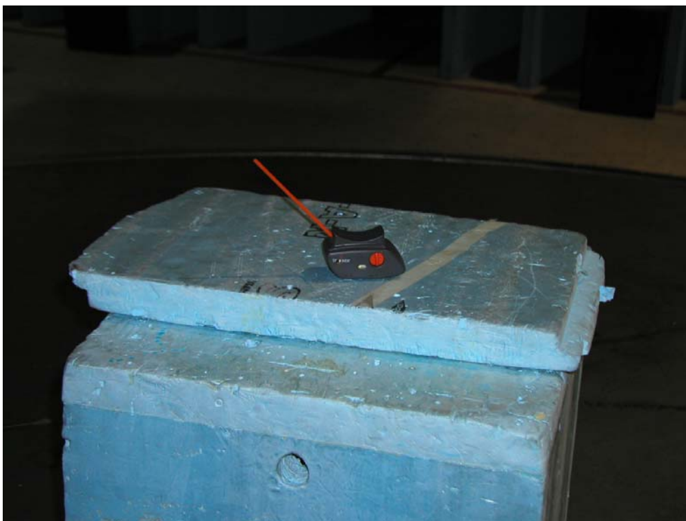
Photograph 3. Radiated RF output power and spurious radiated emissions test setup
