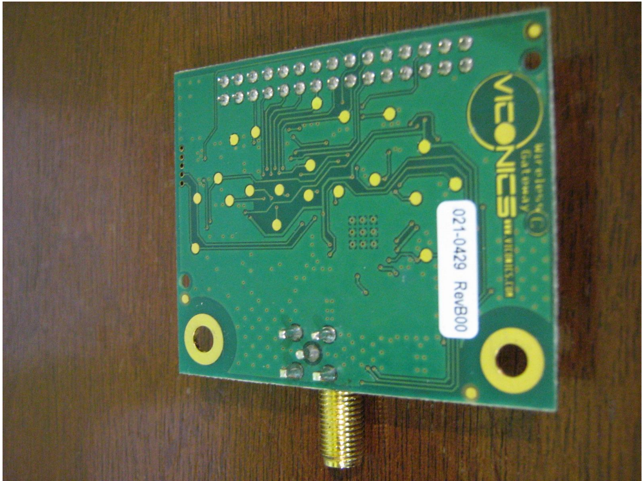
Figure 3 – Solder side RF Chip
