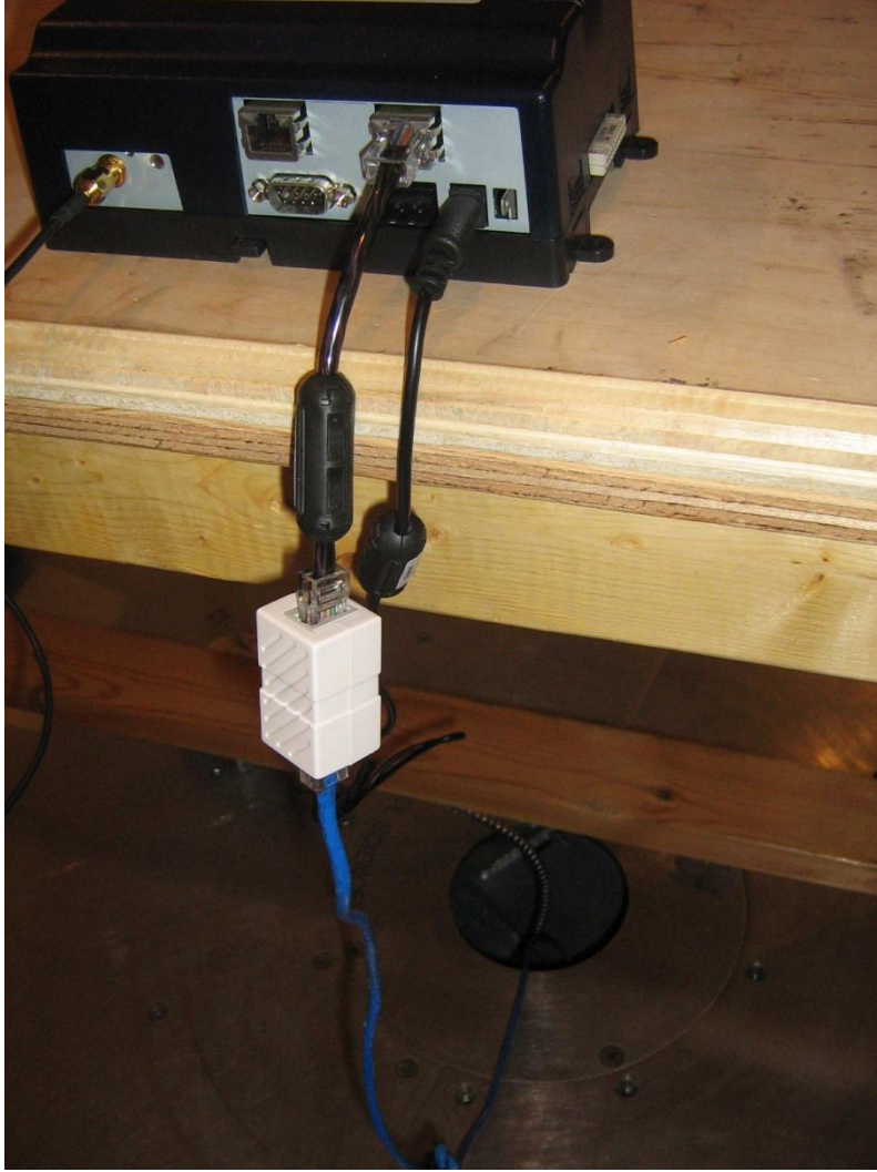
Figure 5 – Ferrites used for compliance
