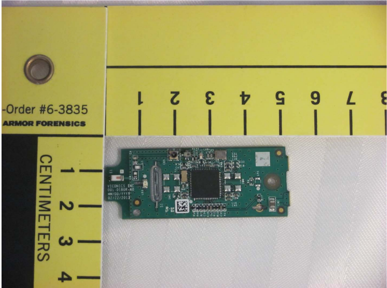
Figure 1: VWAP – front view
