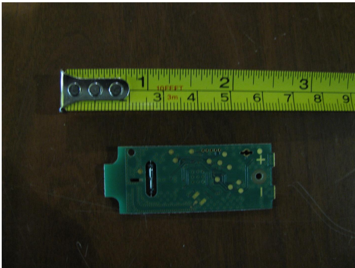
Figure 2 – EUT PCB bottom
