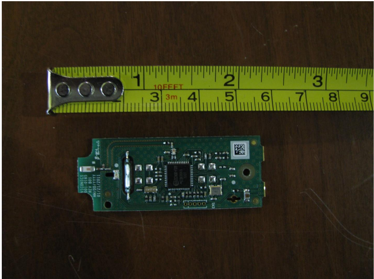
Figure 3 – EUT PCB top
