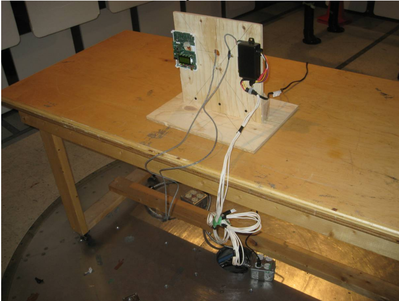
Radiated Emissions Photo 1 (Grantee's Host Configuration)
