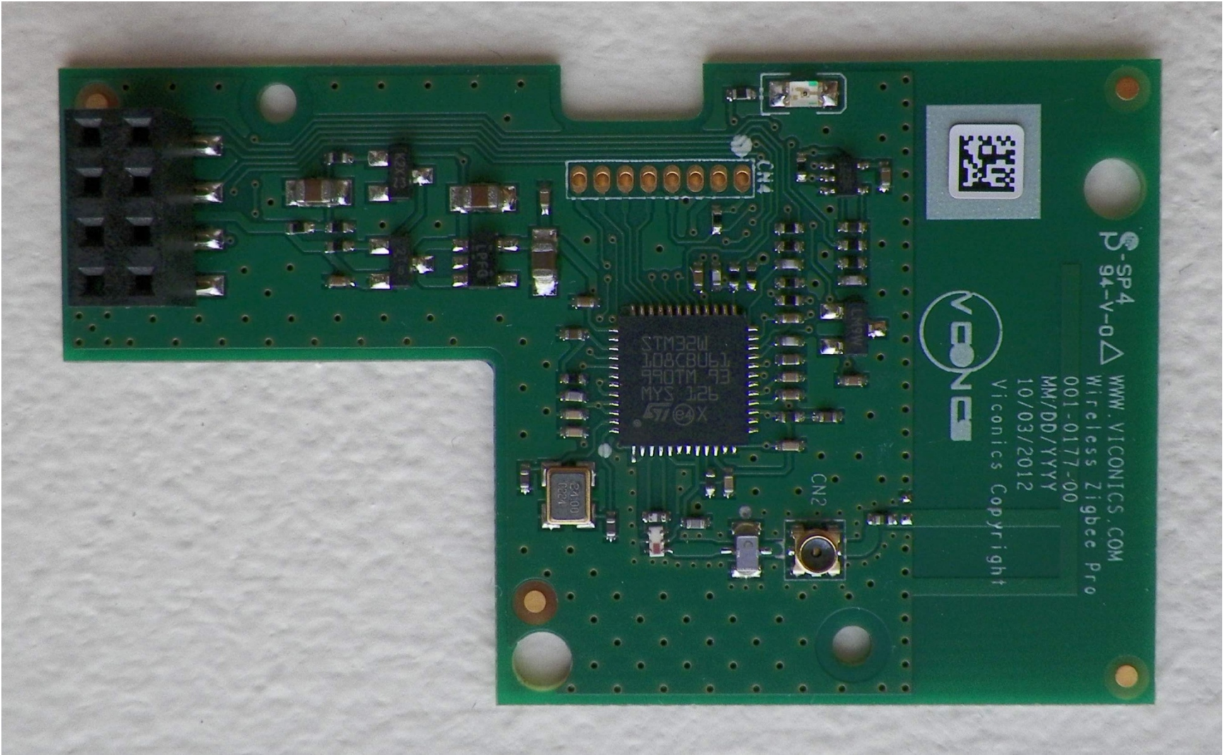
Front (module)
