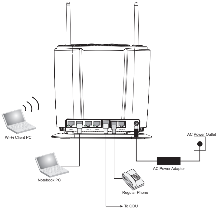
Figure 2-1 IDU Connections
