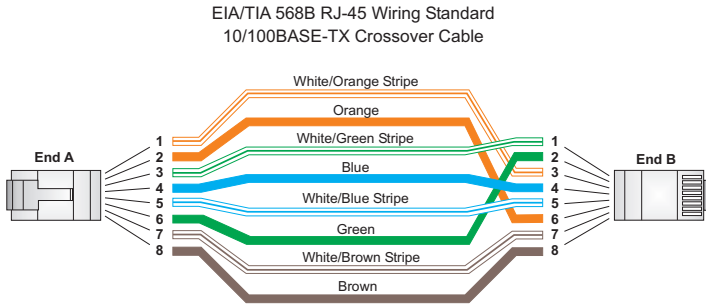
Figure C-3 Crossover Wiring
