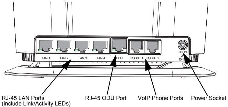
Figure 1-3 Back of the IDU
