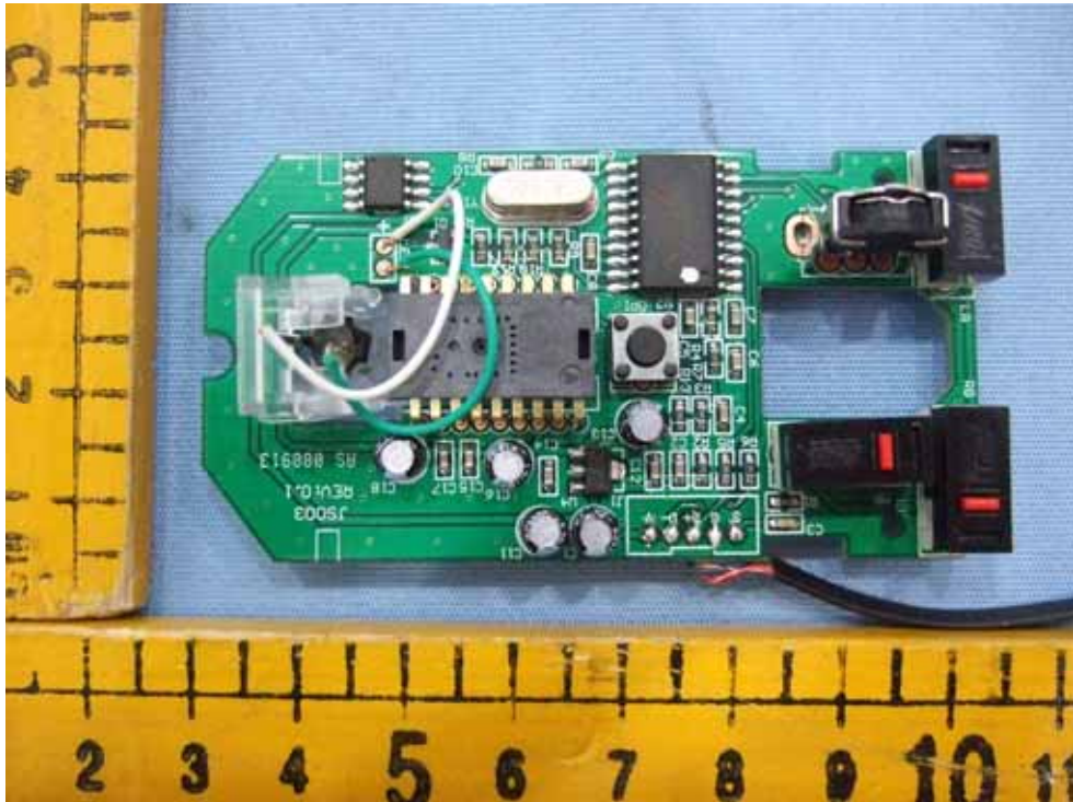
Figure 4 PCB of the EUT-Front View
