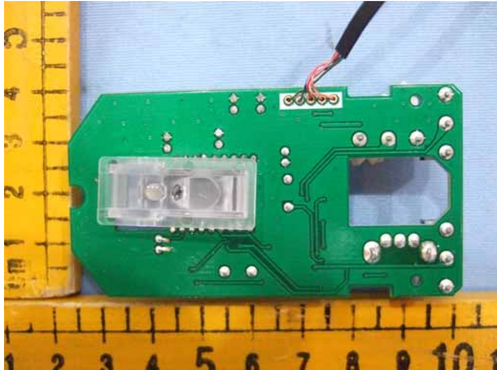
Figure 5 PCB of the EUT -Back View
