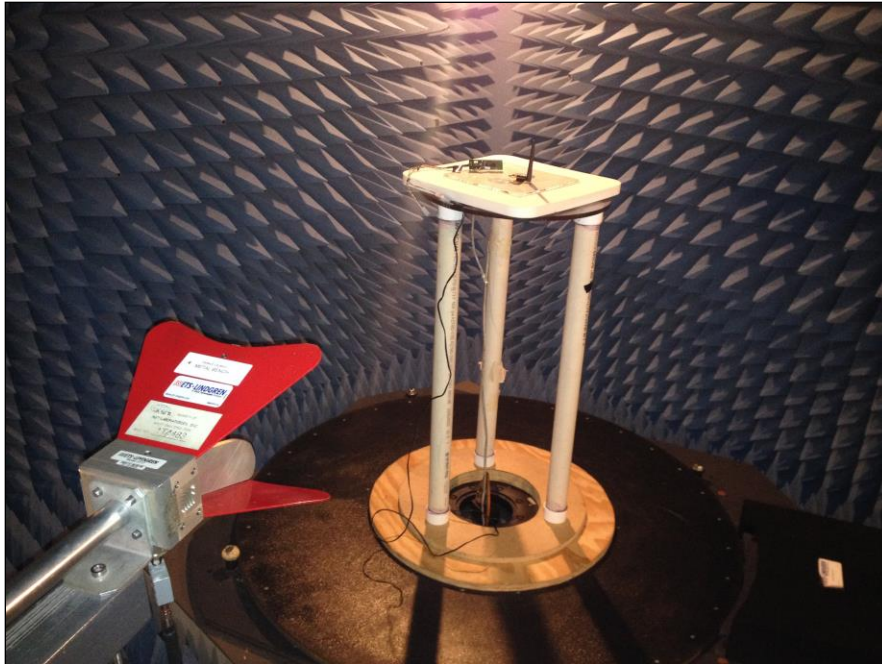
Photograph 7. Radiated Spurious Emissions, Test Setup, External Whip Antenna, 1 GHz – 18 GHz at 1.0m Distance
