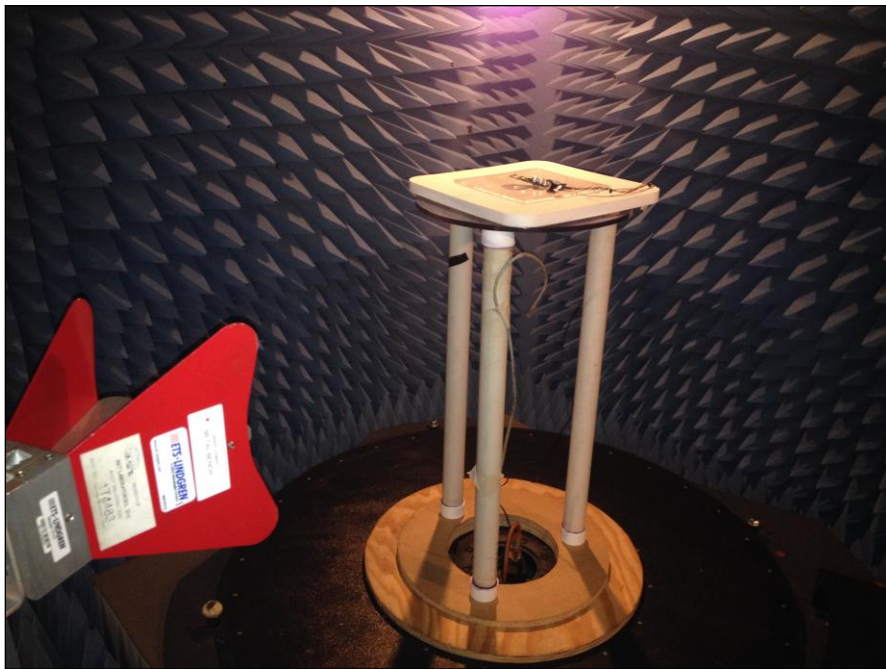
Photograph 5. Radiated Spurious Emissions, Test Setup, Integral Antenna, 1 GHz – 18 GHz at 1.0m Distance
