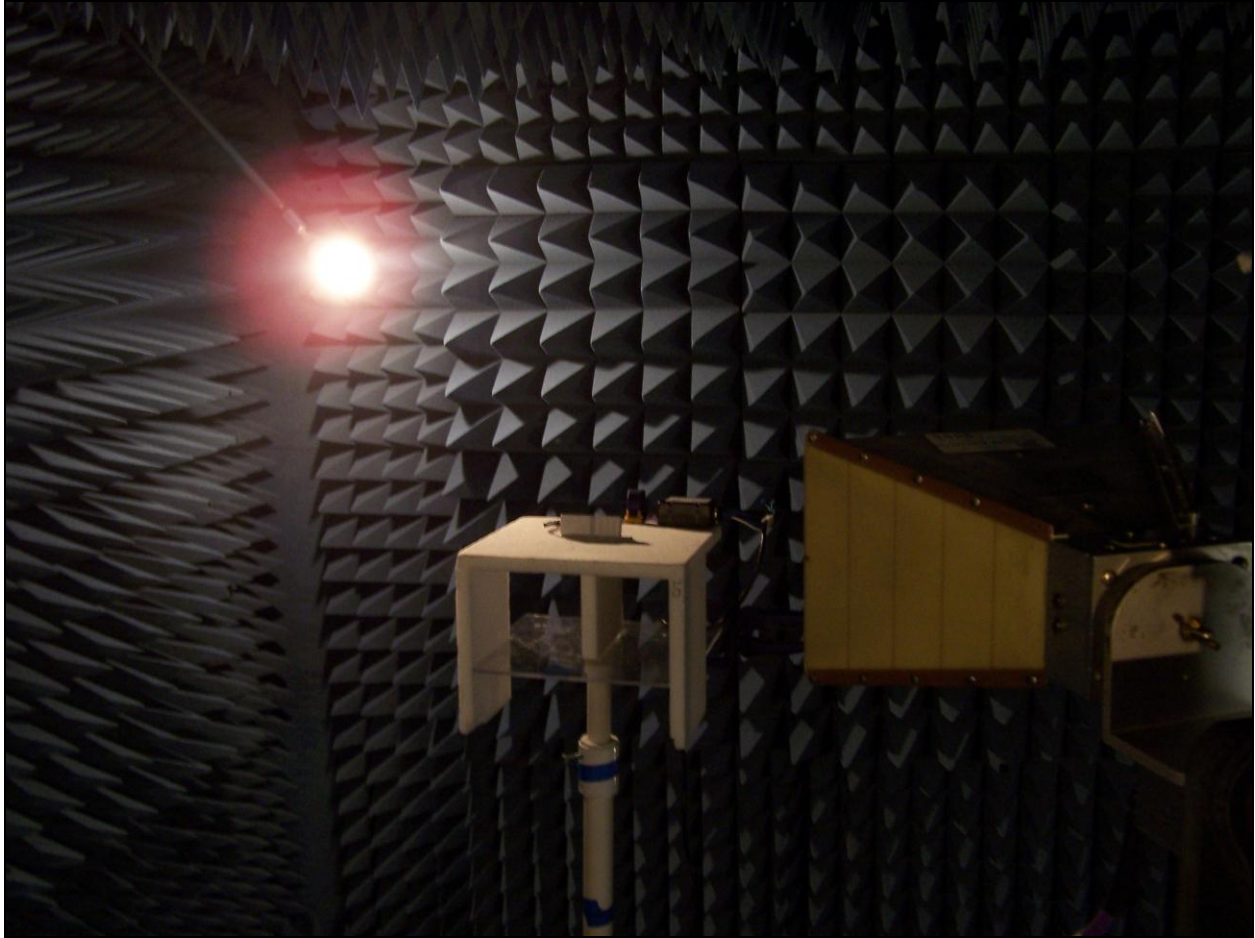
Photograph 1. Radiated Spurious Test Setup
