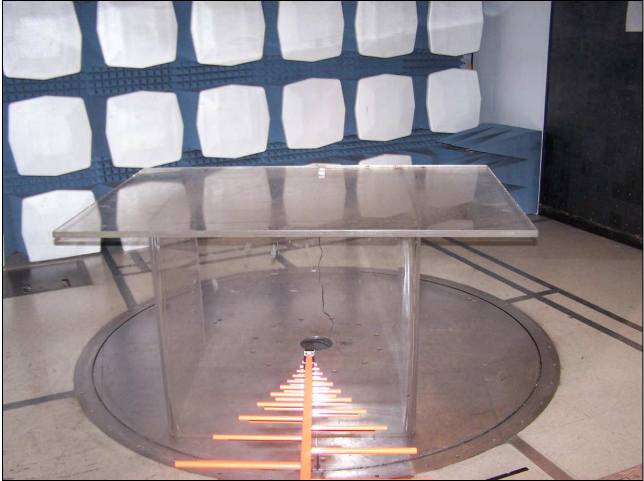
Photograph 3. RE Test Setup, RS232
