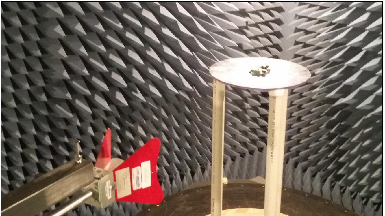
Photograph 4. Radiated Spurious Emissions, Test Setup
