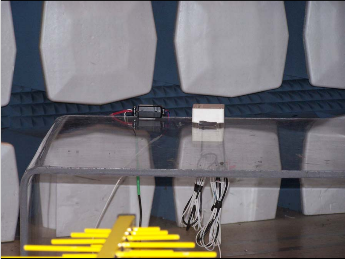
Photograph 6. Radiated Emissions Test Setup
