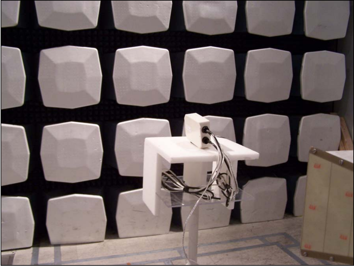
Photograph 5. Harmonics Test Setup
