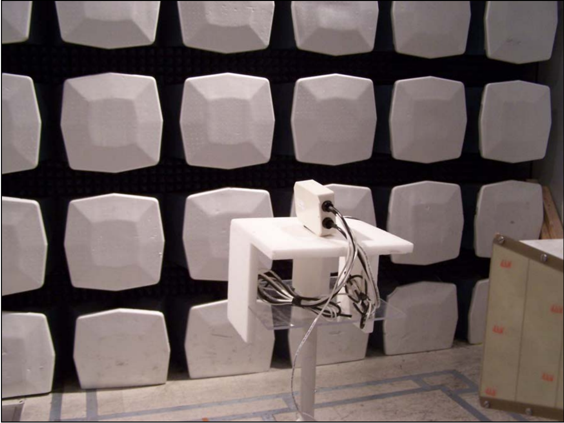
Photograph 4. Power Spectral Density Test Setup
