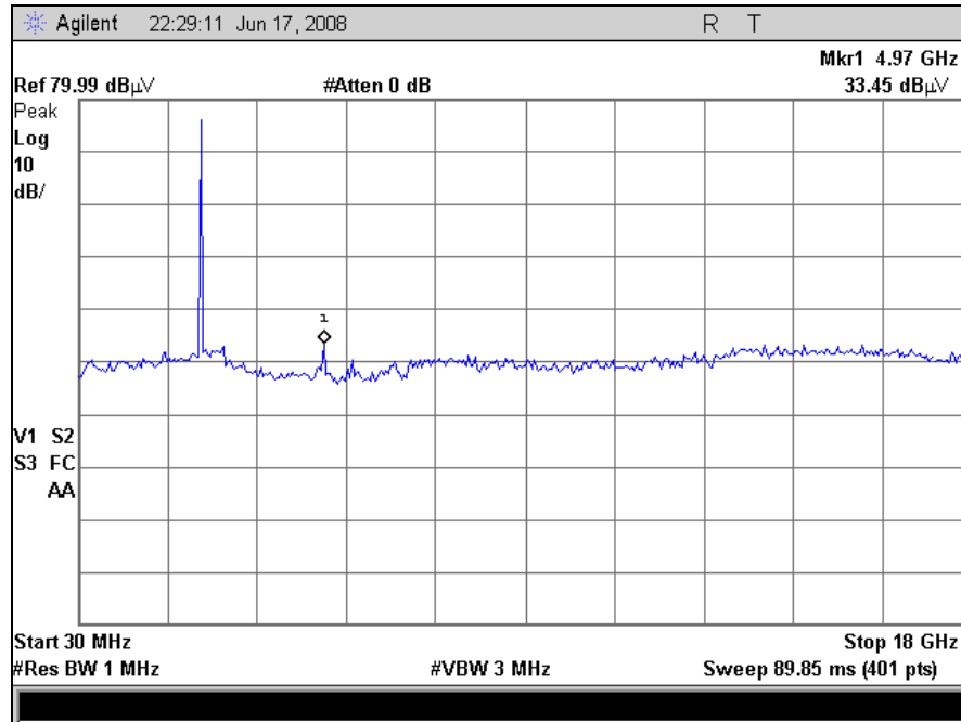
Plot 11. Radiated Spurious, Channel 26
