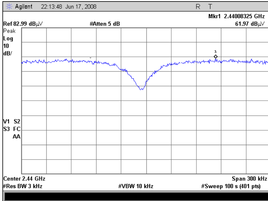
Plot 17. Peak Power Spectral Density, Channel 18
