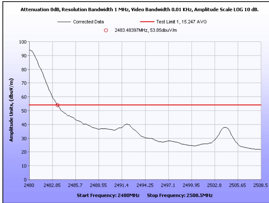
Plot 14. Radiated Restricted Band, Channel 26, Average
