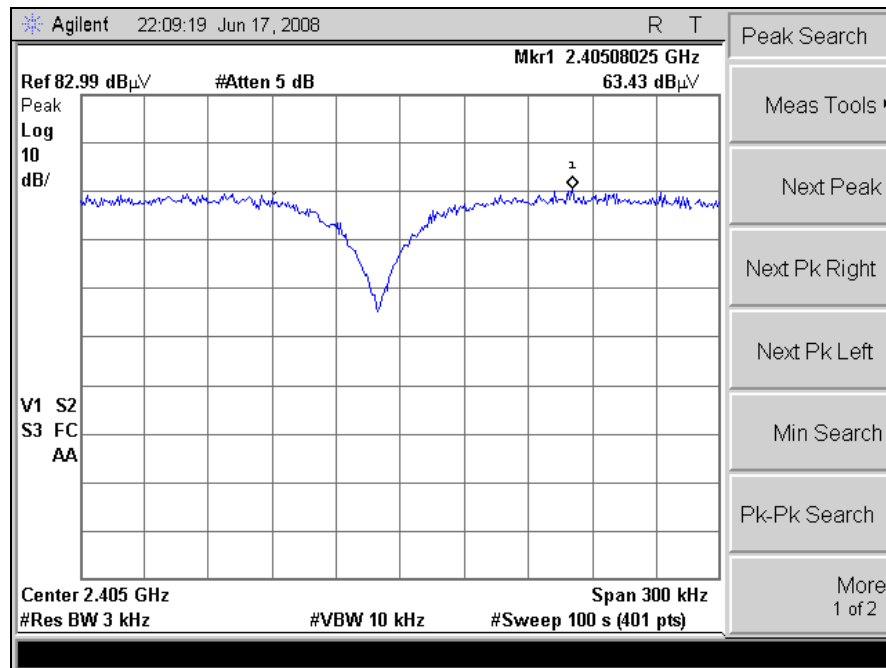
Plot 16. Peak Power Spectral Density, Channel 11
