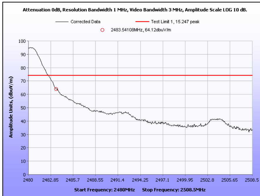
Plot 15. Radiated Restricted Band, Channel 26, Peak
