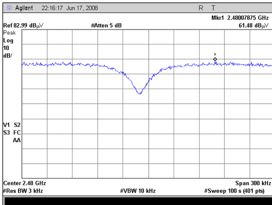
Plot 18. Peak Power Spectral Density, Channel 26
