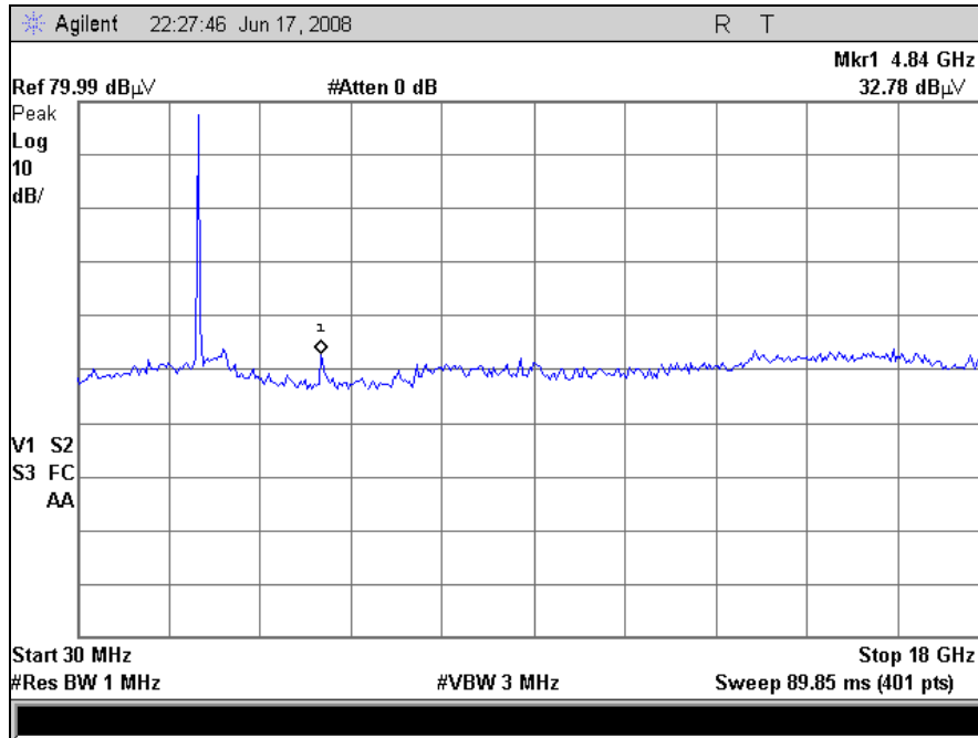
Plot 9. Radiated Spurious, Channel 11
