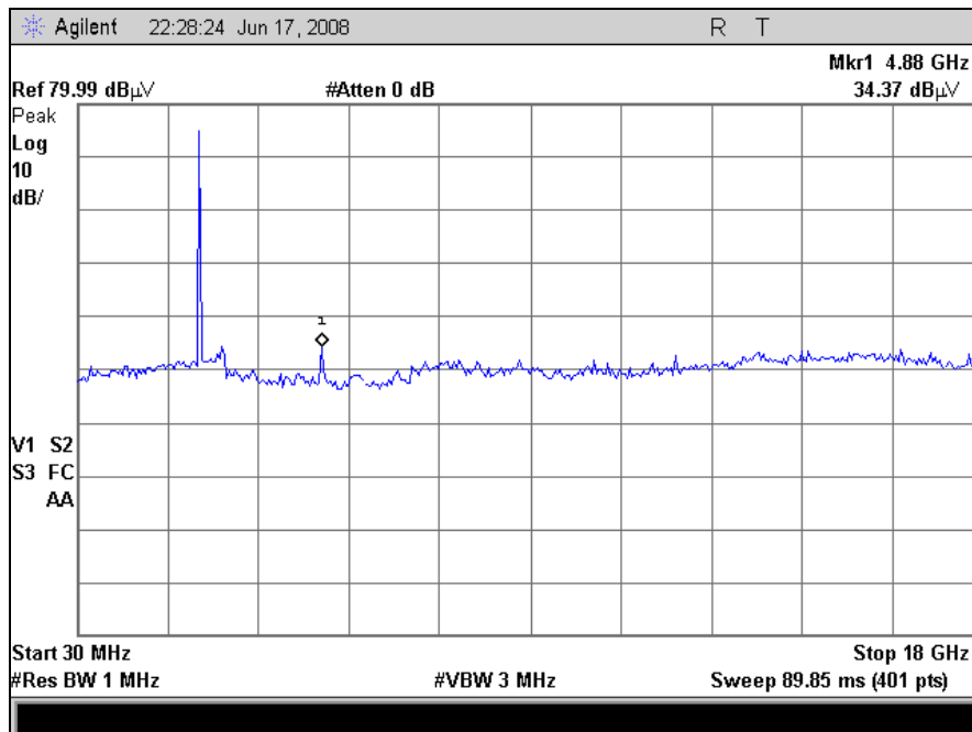
Plot 10. Radiated Spurious, Channel 18
