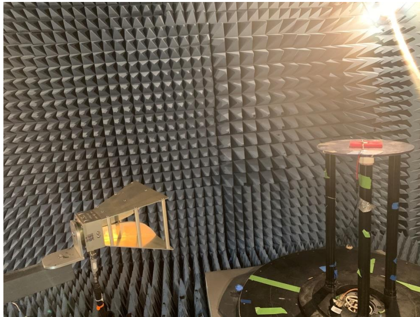
Figure 3: Radiated Spurious Emissions, 1 GHz – 18 GHz, Test Setup
