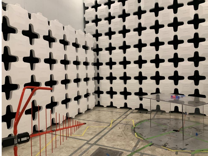
Figure 2: Radiated Spurious Emissions, 30 MHz – 1 GHz, Test Setup
