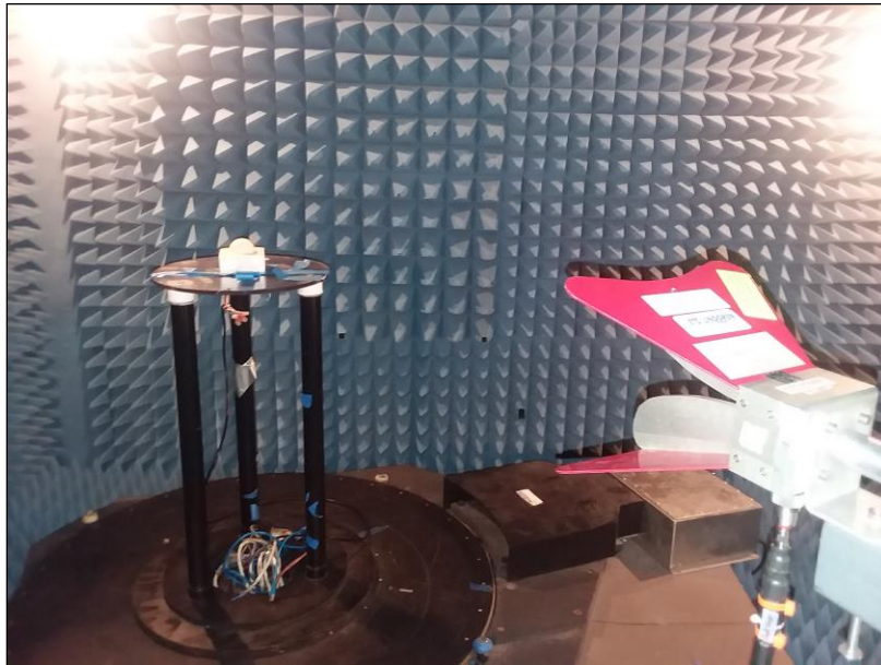
Photograph 3. Radiated Spurious Emissions, Test Setup, Above 1GHz
