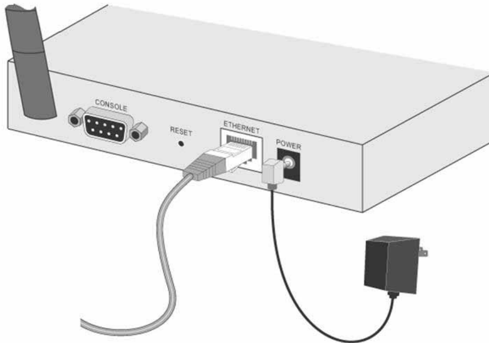
Figure 4: Installation Diagram
