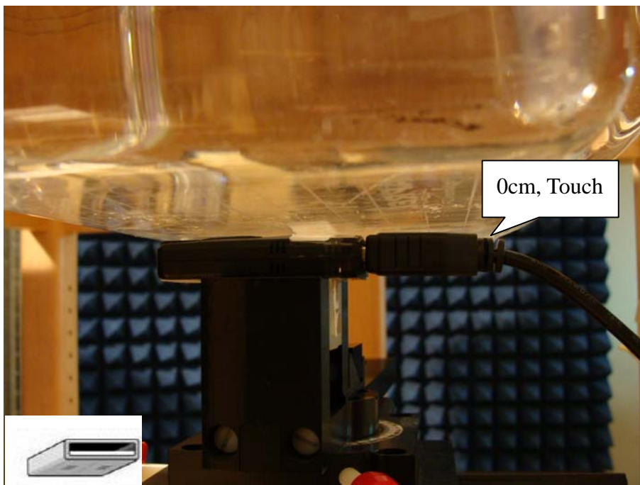
Horizontal-Down EUT connected with NB via USB cable
