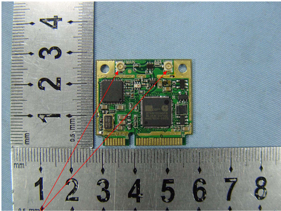
Antenna connector
