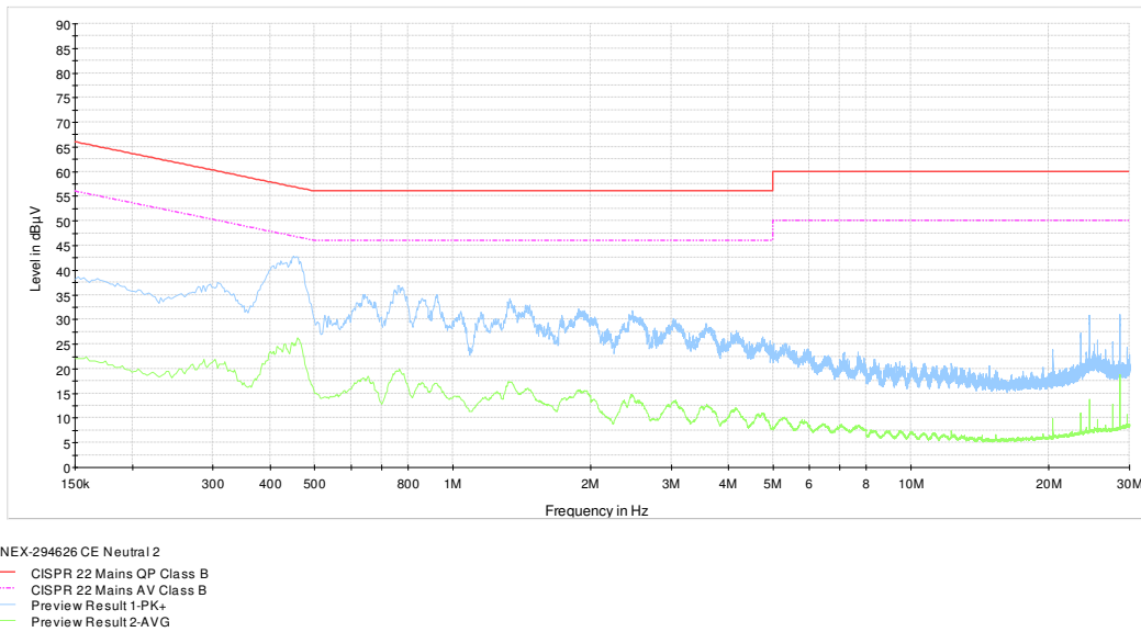
Figure 8.1-4: Conducted disturbance at mains port spectral plot on neutral line Model Clearlink RI
