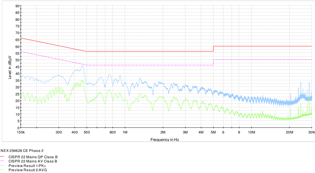
Figure 8.1-3: Conducted disturbance at mains port spectral plot on phase line Model Clearlink RI
