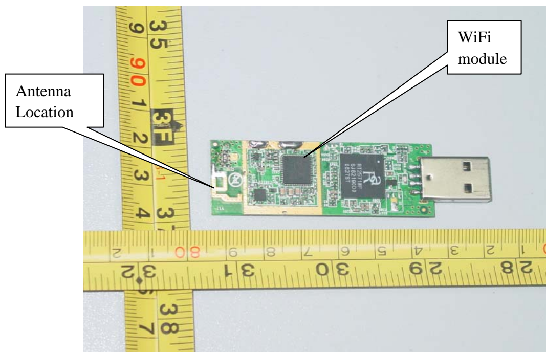
Figure 2 Internal photo of PCB
