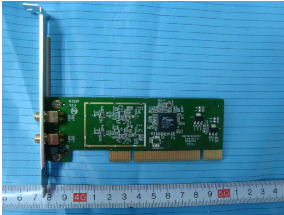
EUT – Main Board without Shielded-Cover TopView
