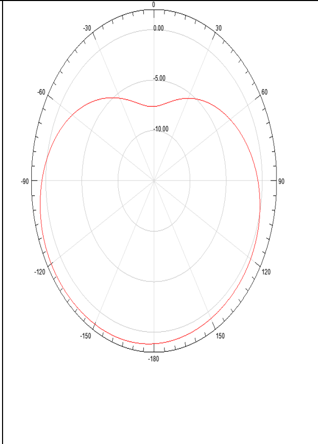
2D radiation pattern (5.5G) H-plane
