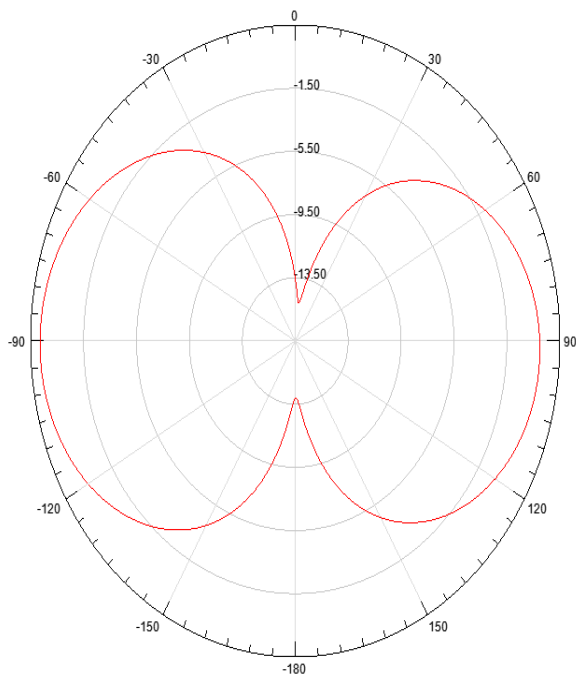
2D radiation pattern (2.4G) V-plane
