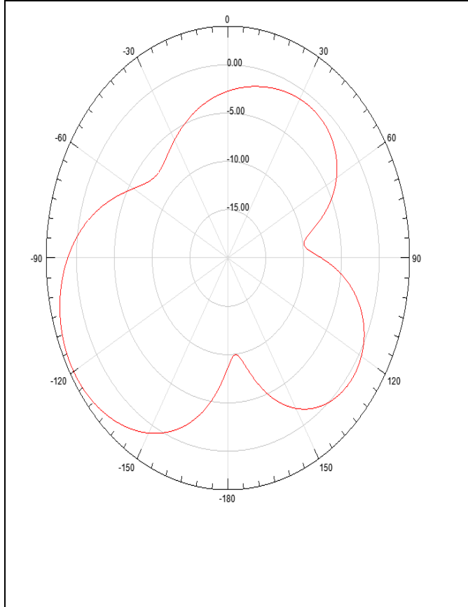
2D radiation pattern (5.5G) V-plane
