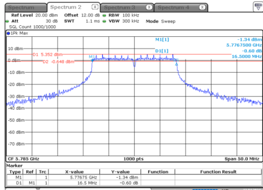
a_5785MHz_Chain 0
