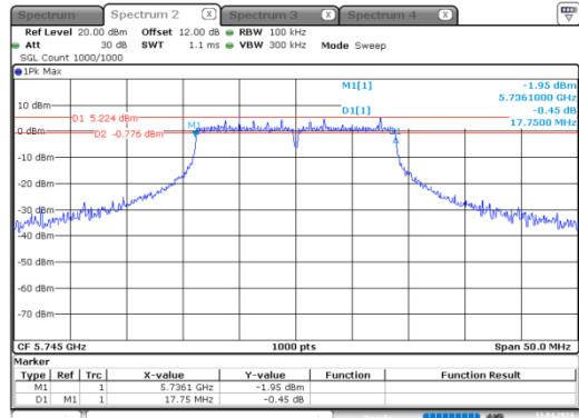
n20_5745MHz_Chain 0
