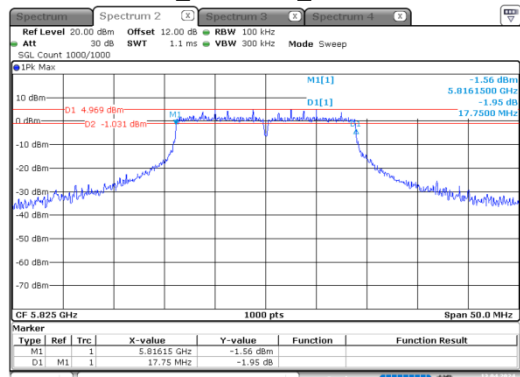
n20_5825MHz_Chain 0
