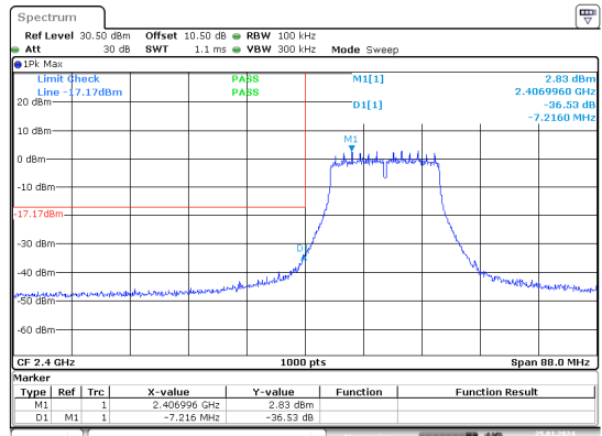
g_2412MHz_Chain 1
