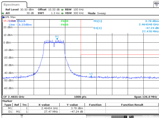
g_2462MHz_Chain 0
