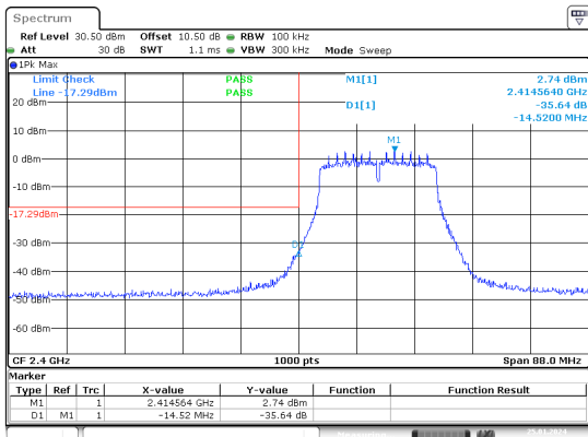
n20_2412MHz_Chain 0
