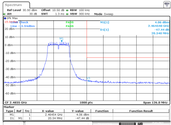
g_2462MHz_Chain 1
