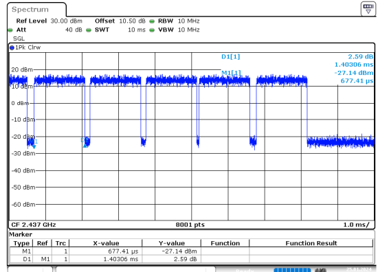
g_2437MHz_Chain 0
