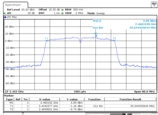
n40_2452MHz_Chain 0
