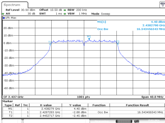
g_2437MHz_Chain 0
