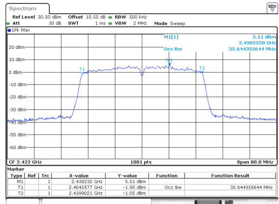
n40_2422MHz_Chain 0
