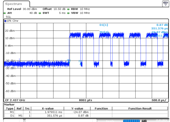
n40_2437MHz_Chain 0
