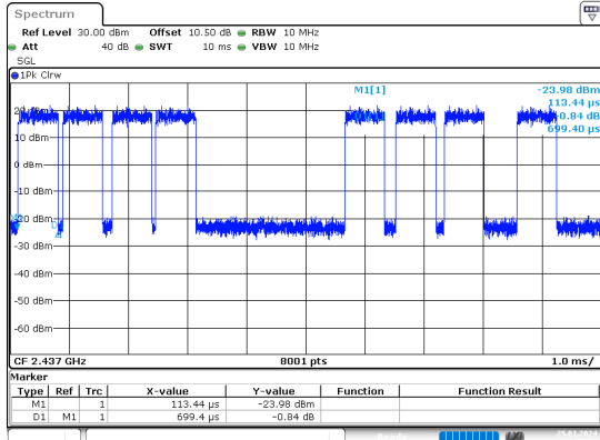
n20_2437MHz_Chain 0
