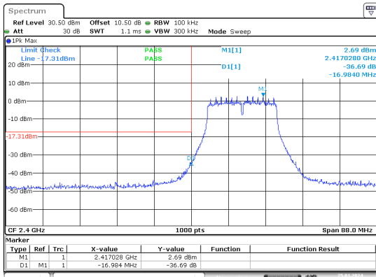
g_2412MHz_Chain 0
