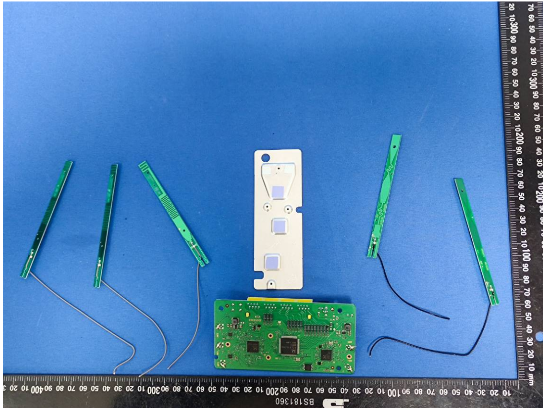
5G Antenna
