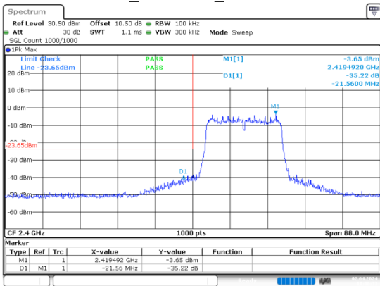
n20_2412MHz_Chain 0
