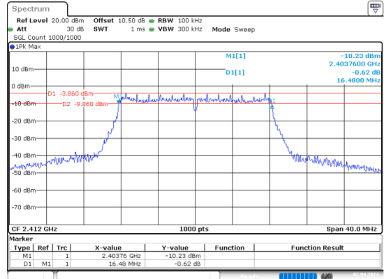
g_2412MHz_Chain 0
