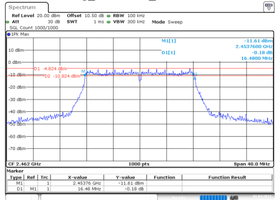
g_2462MHz_Chain 0
