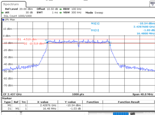
g_2437MHz_Chain 0
