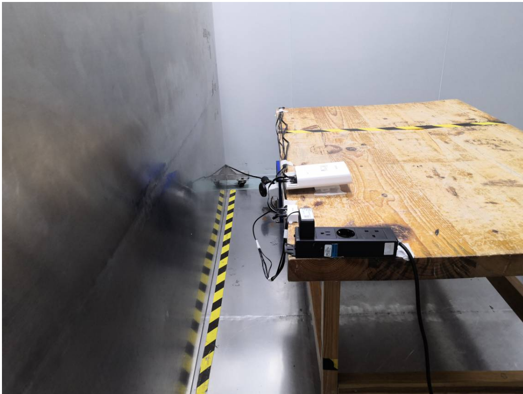
Conducted Emissions Side View-PoE Power Mode
