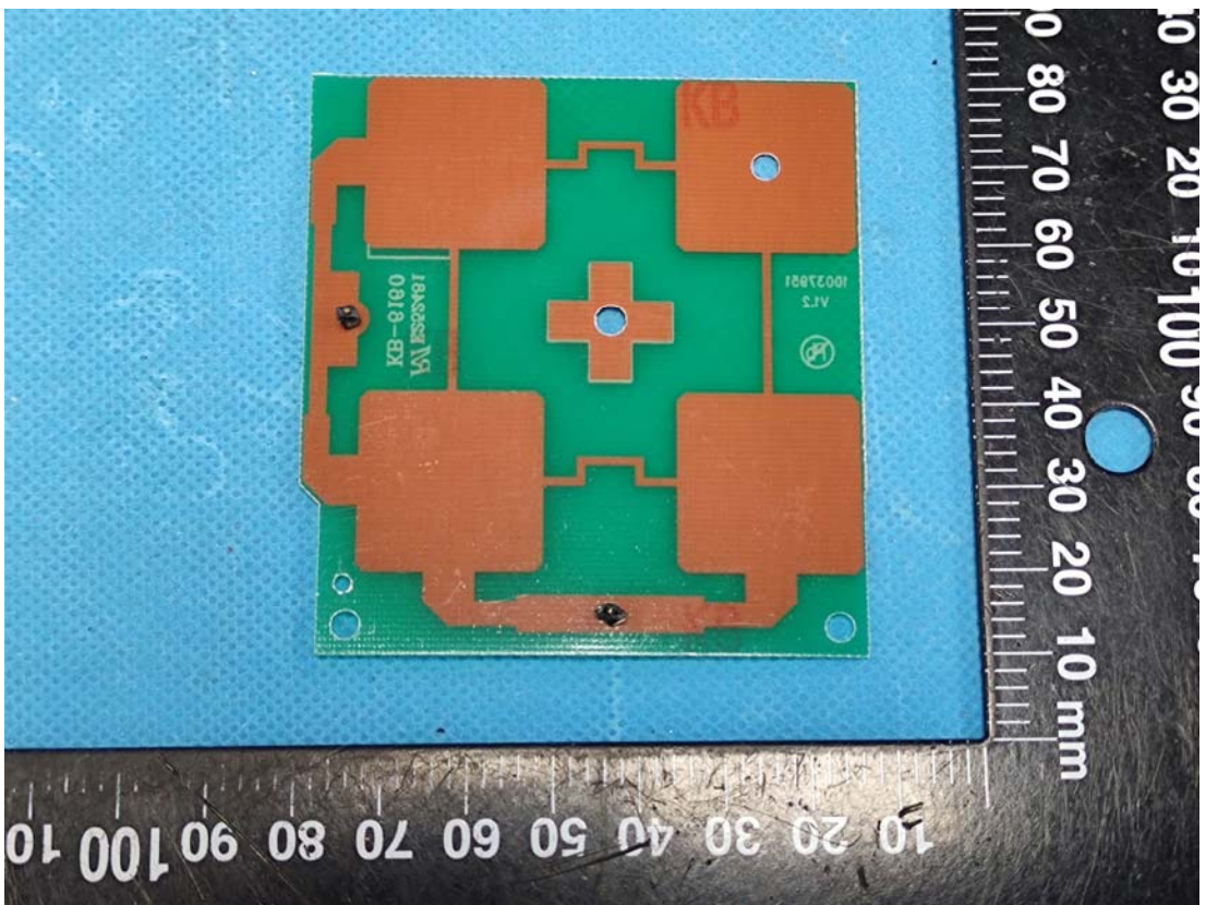
Antenna Chain 1
