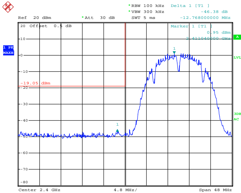
Chain 0, 802.11b: Band Edge, Left Side
