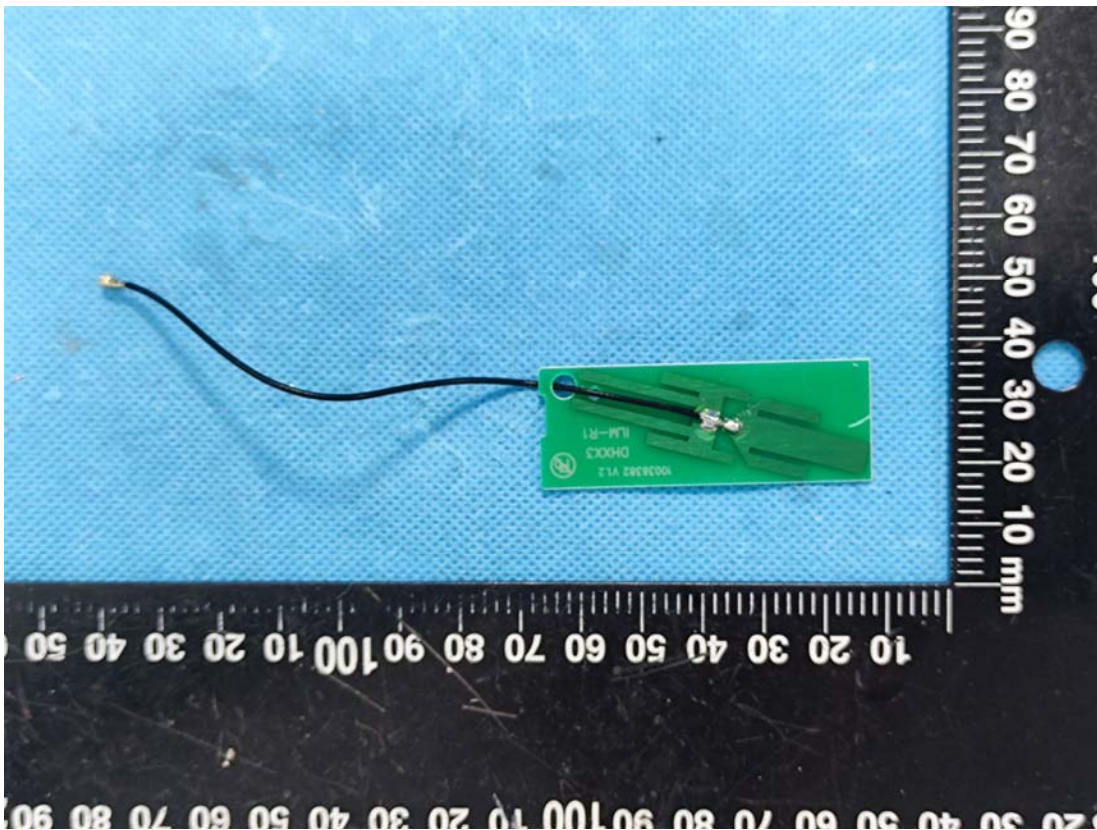
Antenna Chain 0
