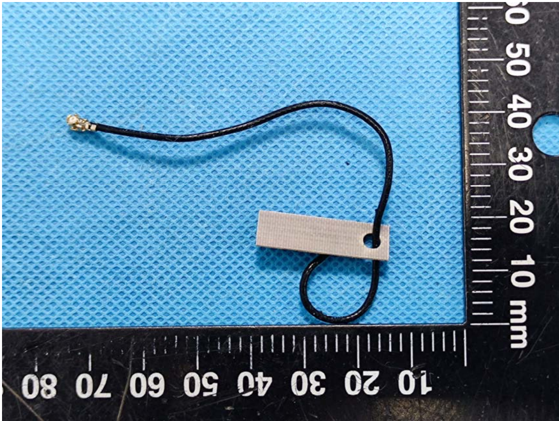
5G Antenna Chain 1
