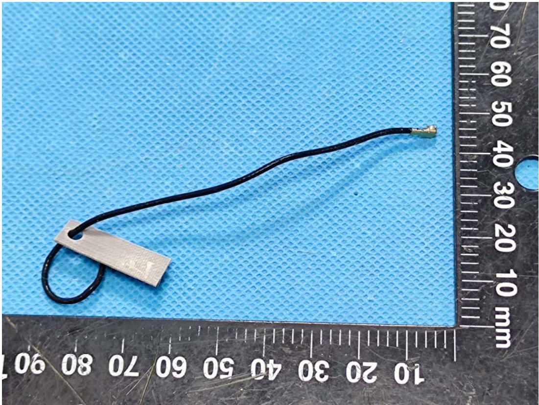
5G Antenna Chain 3
