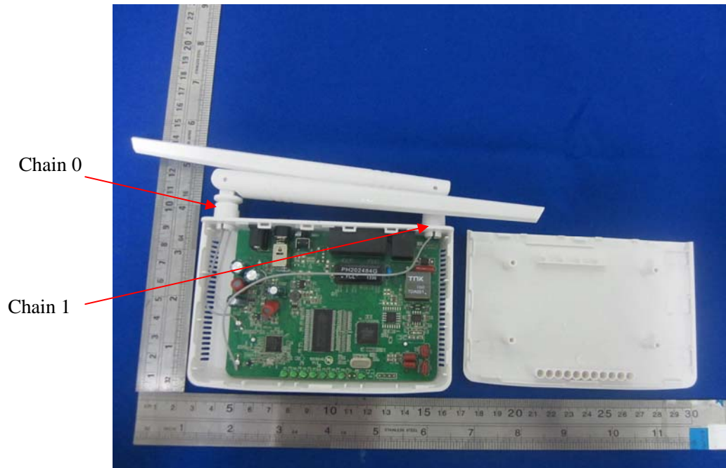
EUT-Uncover View
