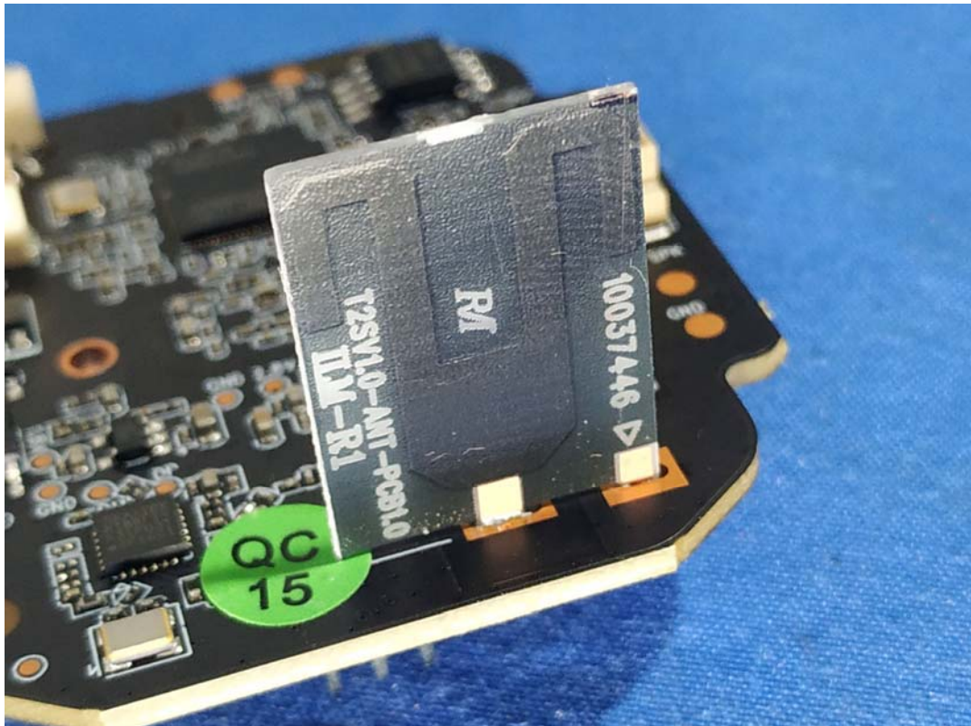
Antenna Board
