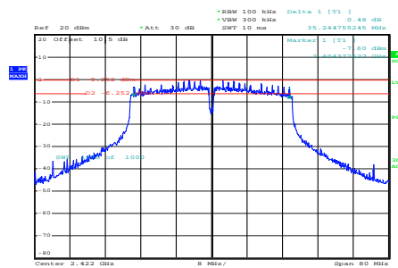
n40_2422MHz_Chain 0
