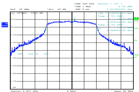
g_2437MHz_Chain 0
