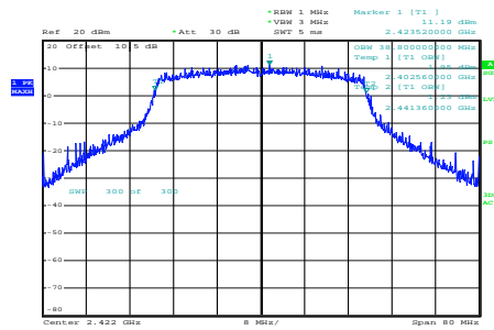
ax40_2422MHz_RU_Full_Chain 0
