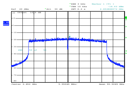
ax40_2452MHz_RU_Full_Chain 0
