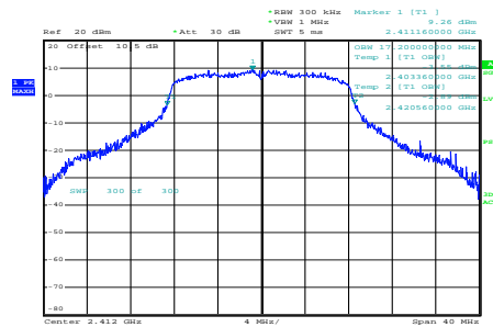
g_2412MHz_Chain 0
