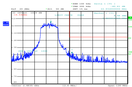
ax20_2462MHz_RU_Full_Chain 0
