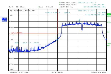
n40_2422MHz_Chain 0
