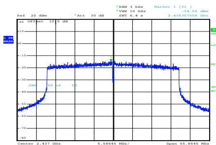
ax40_2437MHz_RU_Full_Chain 0
