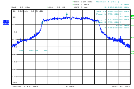
ax20_2437MHz_RU_Full_Chain 0
