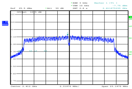
n20_2412MHz_Chain 0
