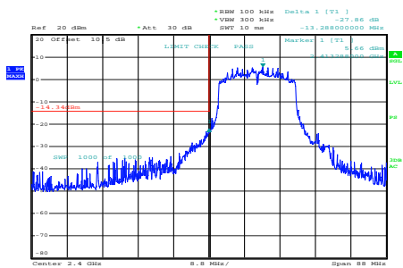
ax20_2412MHz_RU_Full_Chain 0
