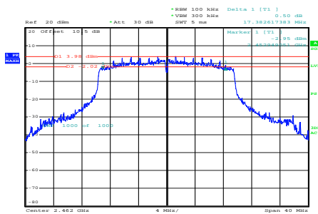
ax20_2462MHz_RU_Full_Chain 0
