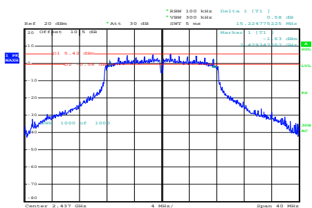
g_2437MHz_Chain 0
