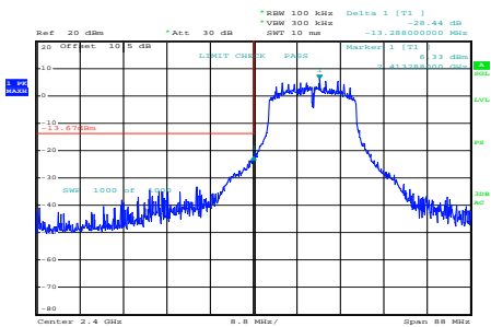
n20_2412MHz_Chain 0
