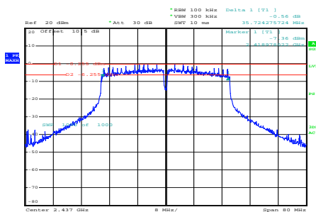
n40_2437MHz_Chain 0
