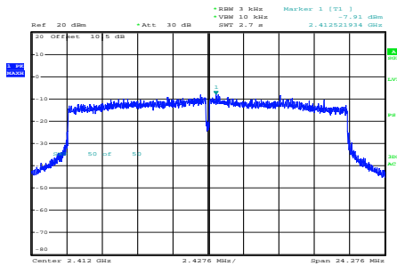
ax20_2412MHz_RU_Full_Chain 0
