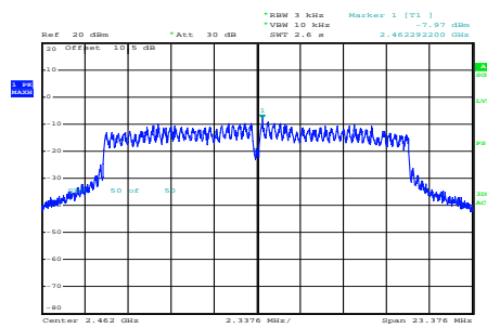
g_2462MHz_Chain 0
