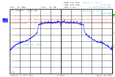
n20_2437MHz_Chain 0
