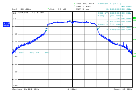
g_2462MHz_Chain 0
