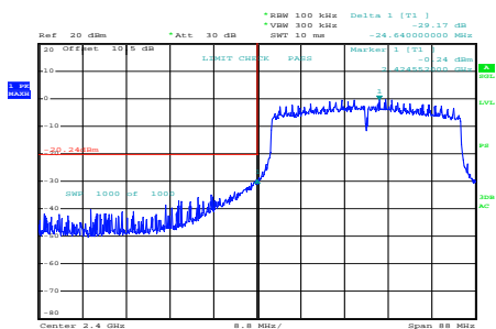
ax40_2422MHz_RU_Full_Chain 0
