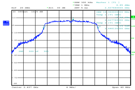
n20_2437MHz_Chain 0
