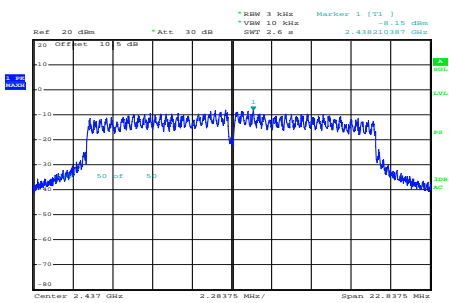
g_2437MHz_Chain 0
