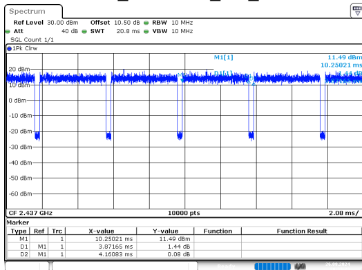
ax20_2437MHz_RU_Full
