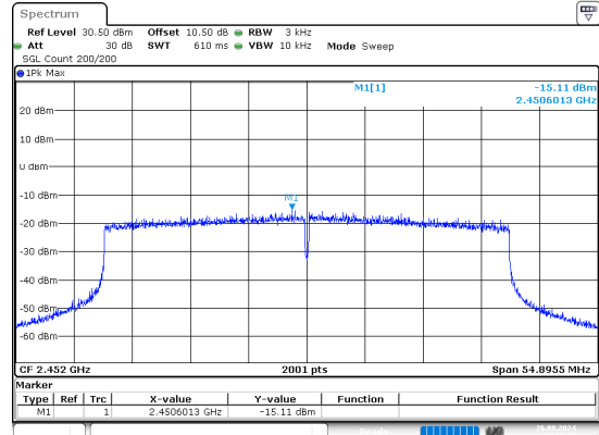
ax40_2452MHz_RU_Full
