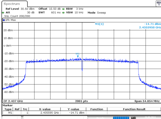
ax40_2437MHz_RU_Full
