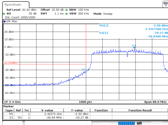
ax40_2422MHz_RU_Full
