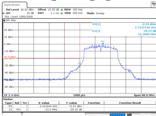
ax20_2412MHz_RU_Full
