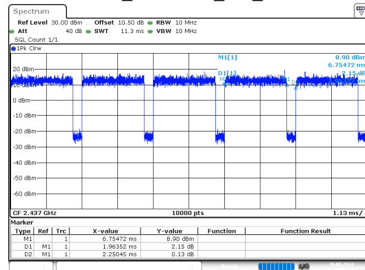
ax40_2437MHz_RU_Full
