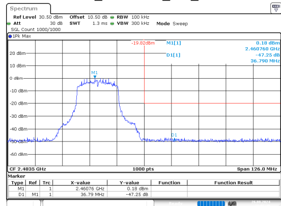
ax20_2462MHz_RU_Full
