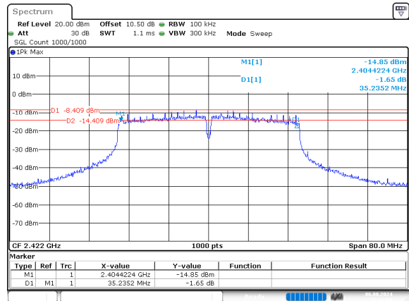
n40_2422MHz
