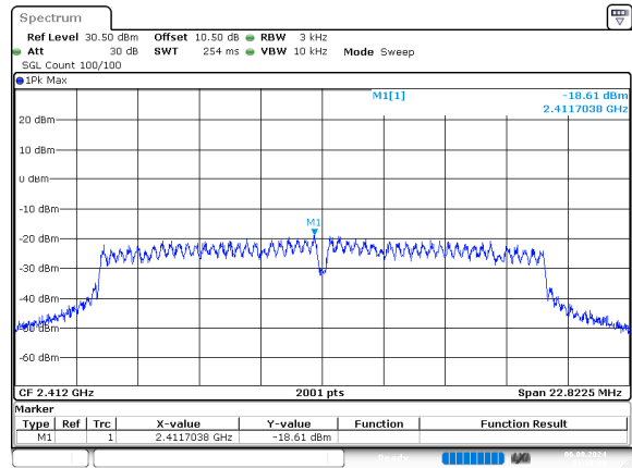
g_2412MHz
