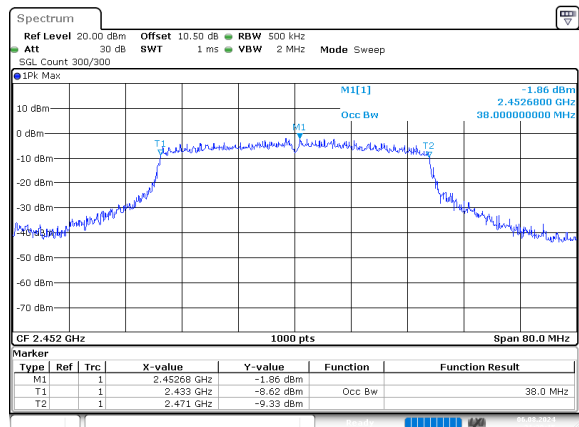
ax40_2452MHz_RU_Full
