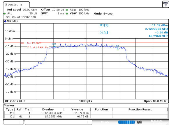
ax20_2437MHz_RU_Full
