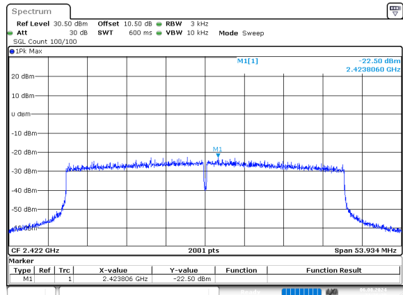
ax40_2422MHz_RU_Full
