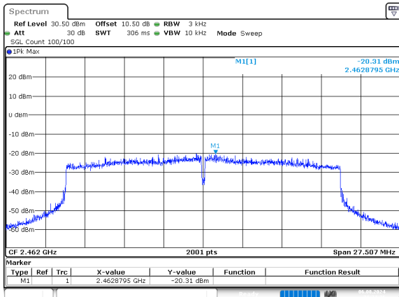
ax20_2462MHz_RU_Full
