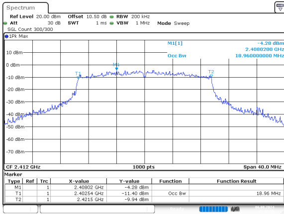
ax20_2412MHz_RU_Full
