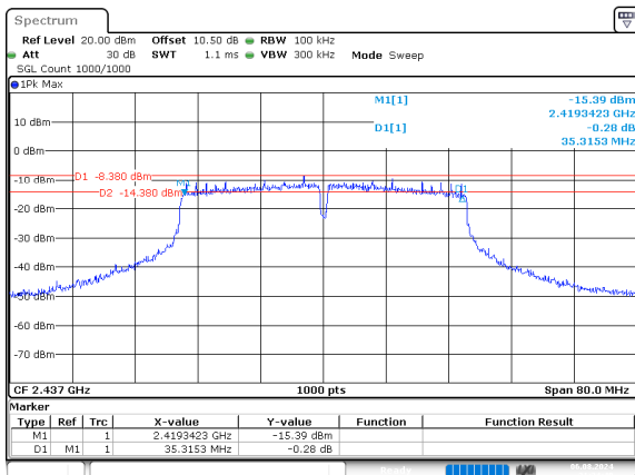
n40_2437MHz
