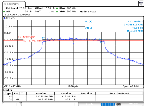
n20_2437MHz
