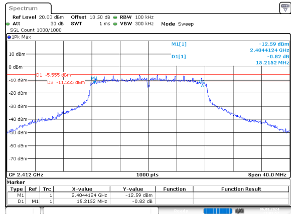
g_2412MHz
