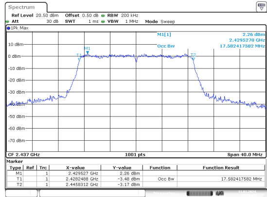
n20_2437MHz_Chain 0
