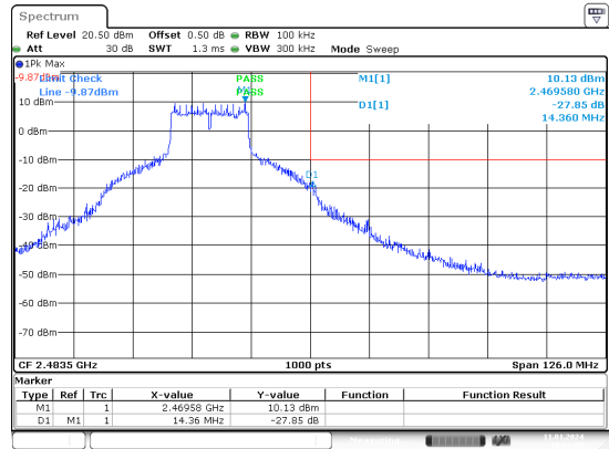
g_2462MHz_Chain 1
