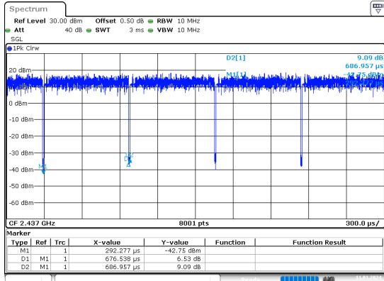
n20_2437MHz_Chain 0
