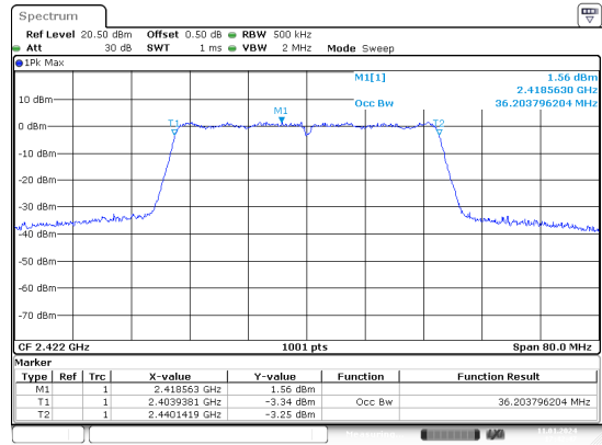
n40_2422MHz_Chain 0
