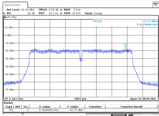
n40_2437MHz_Chain 1
