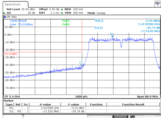
n40_2422MHz_Chain 1
