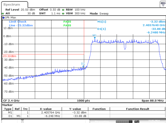
n40_2422MHz_Chain 0
