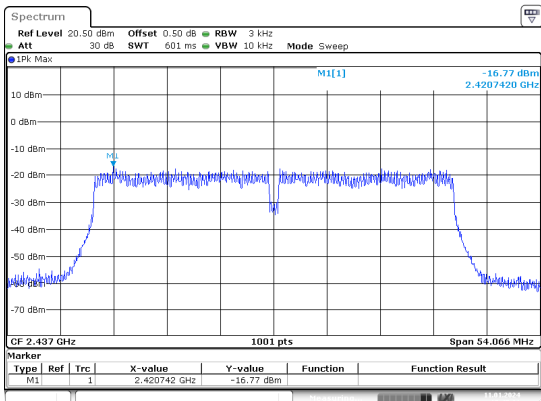
n40_2437MHz_Chain 0
