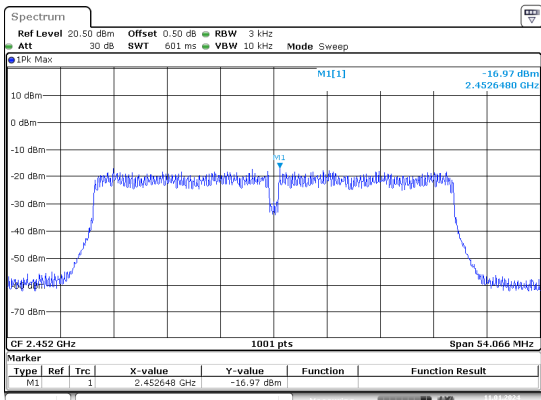
n40_2452MHz_Chain 0
