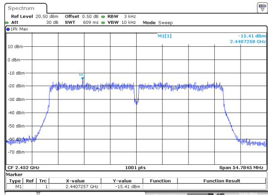
n40_2452MHz_Chain 1
