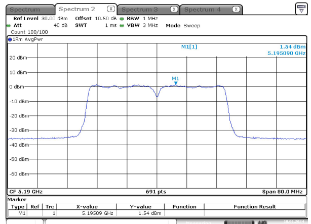
ac40_5190MHz_Chain 1
