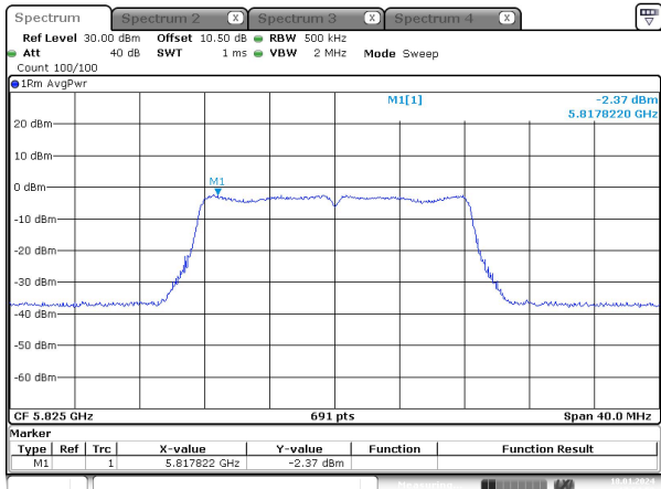
a_5825MHz_Chain 0
