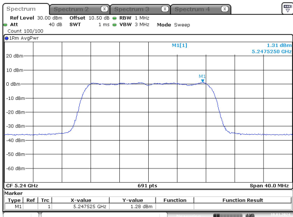
ac20_5240MHz_Chain 1
