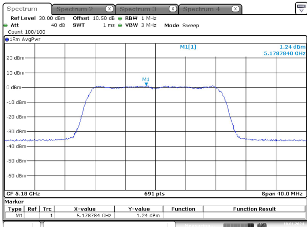
ac20_5180MHz_Chain 1
