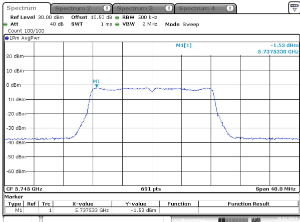
a_5745 MHz_Chain 0
