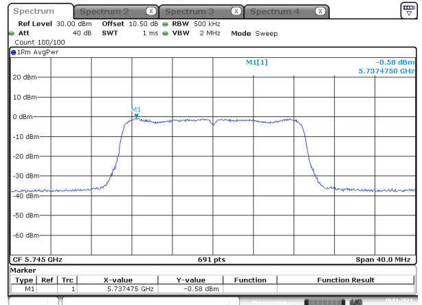
n20_5745MHz_Chain 0
