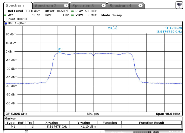
n20_5825MHz_Chain 0
