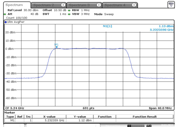
n20_5240MHz_Chain 1
