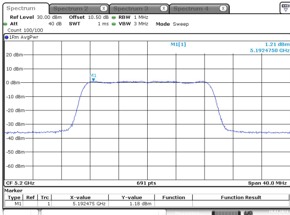
n20_5200MHz_Chain 1
