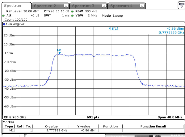
n20_5785MHz_Chain 0
