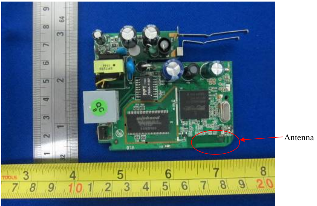
EUT –Main Board with Antenna Top View
