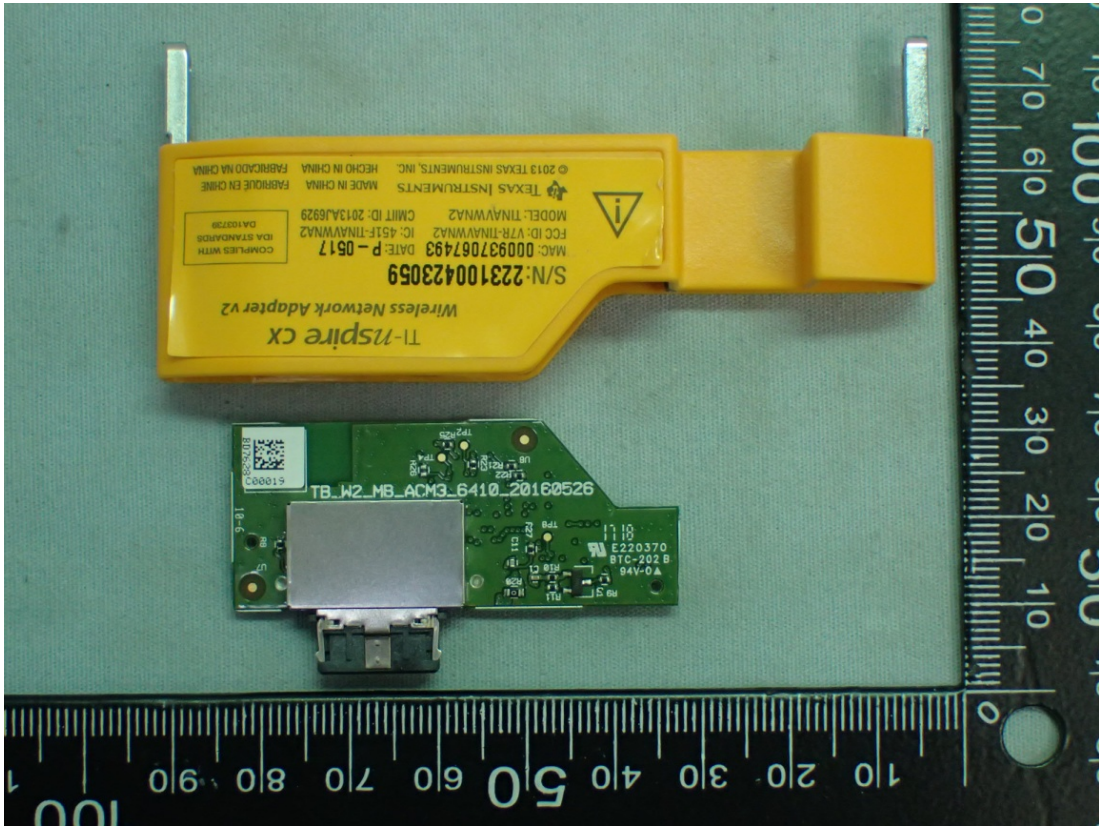
Figure 5 Internal View
